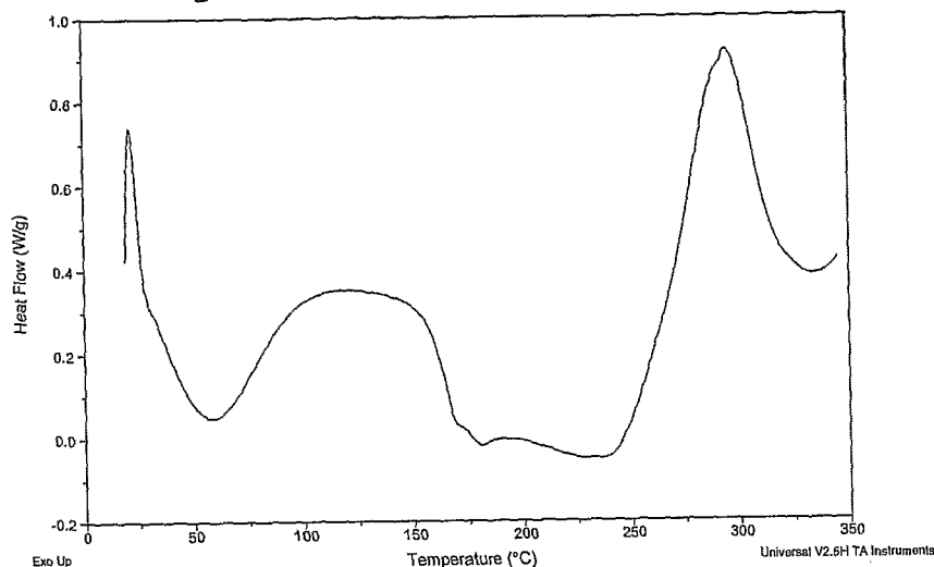
DSC thermogram of amorphous II/PVP (Flash Evaporation)
