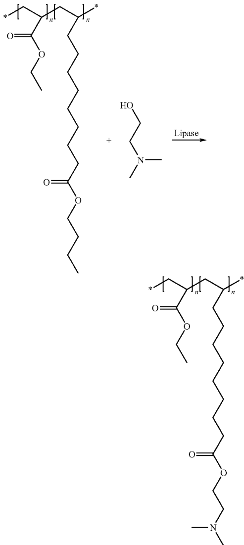
Scheme V
