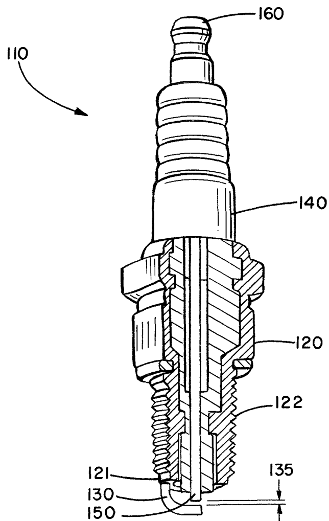
Traditional J-Type Spark Plug
