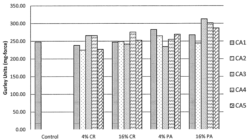
Gurley Stiffness: Method 1, Lab 1
