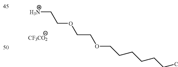
a compound of formula V
