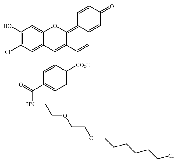
a compound of formula XVIII
