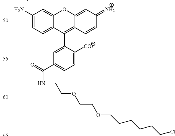
a compound of formula XI
