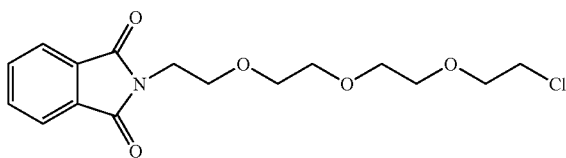
a compound of formula XXVI
