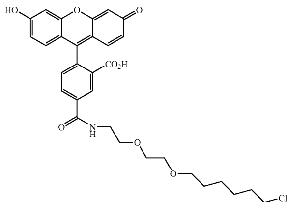
a compound of formula VI
