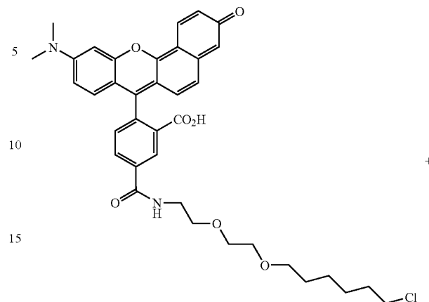
a compound of formula XIX
