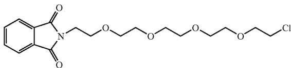
a compound of formula XXVII
