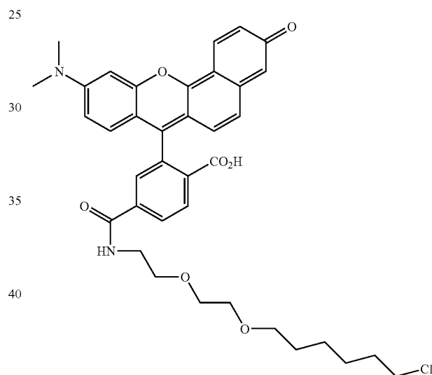
a compound of formula XX
