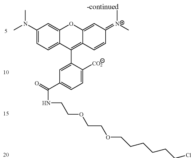
a compound of formula IX
