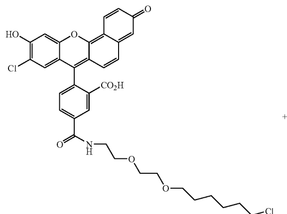
a compound of formula XVII
