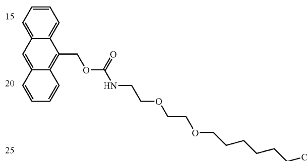
a compound of formula IV
