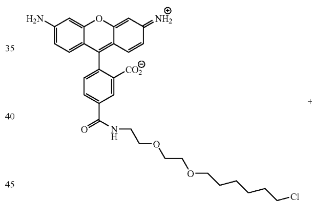
a compound of formula X
