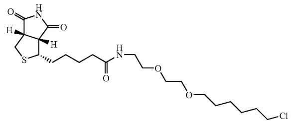
a compound of formula VII
