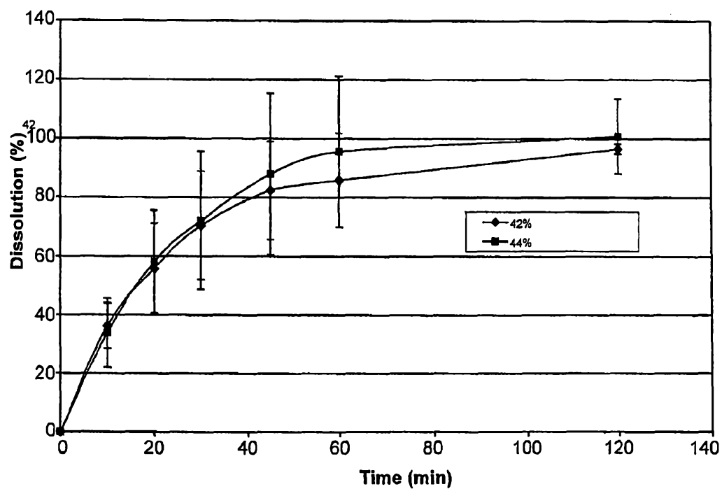
Figure 10 42% and 44% dissolution profile results
