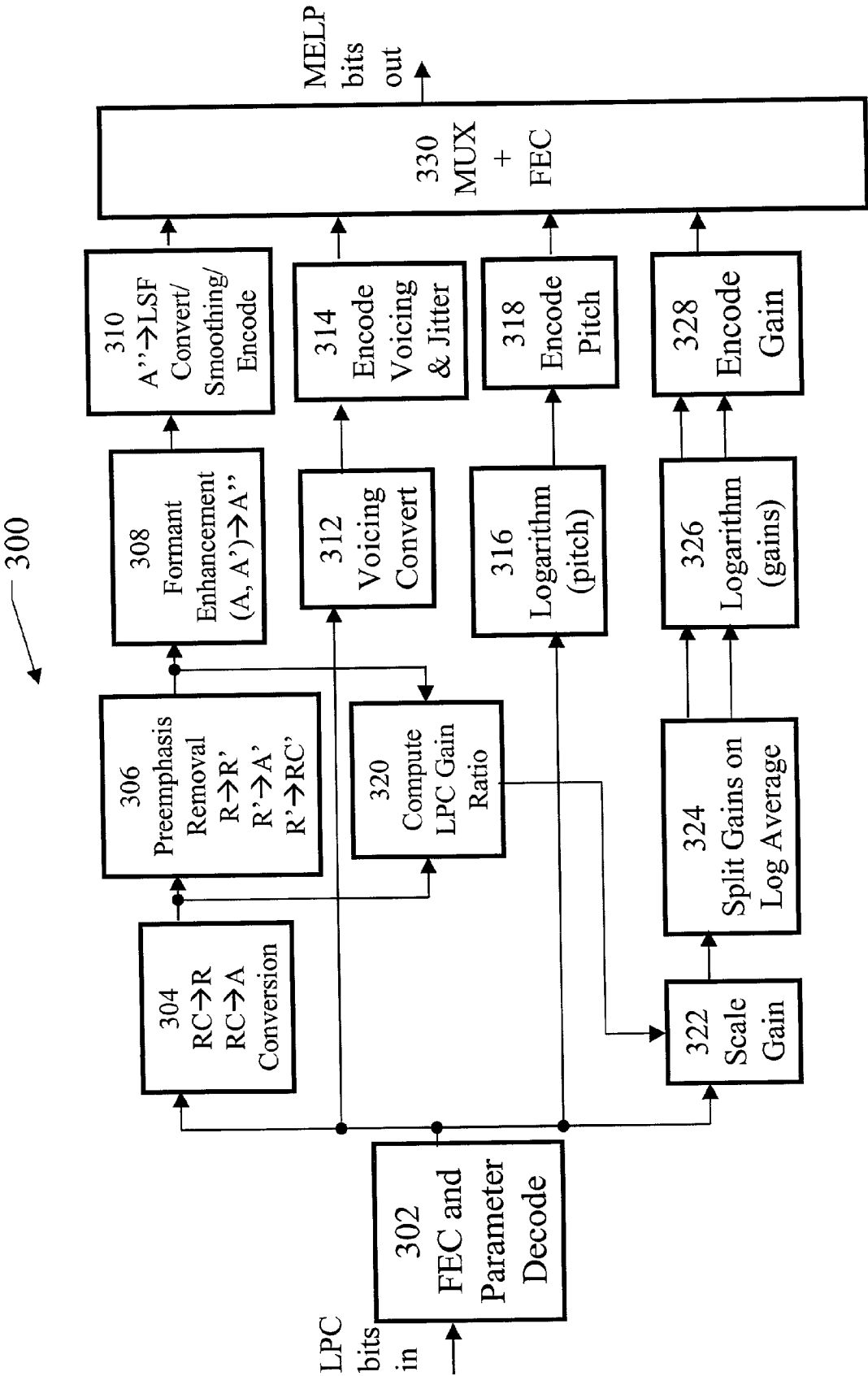
Figure 3: LPC to MELP Transcoder
