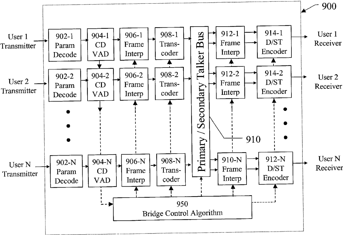
Compressed Domain Conference Bridge
