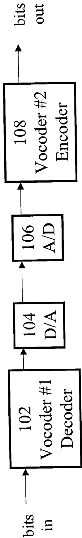
Figure 1: (Prior Art) Tandem Connection
