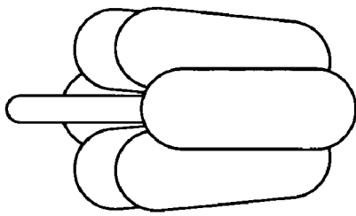
Cartoon of the multi-subunit enzyme - ATPase - that rotates in response to ATP synthesis to hydrolysis.
