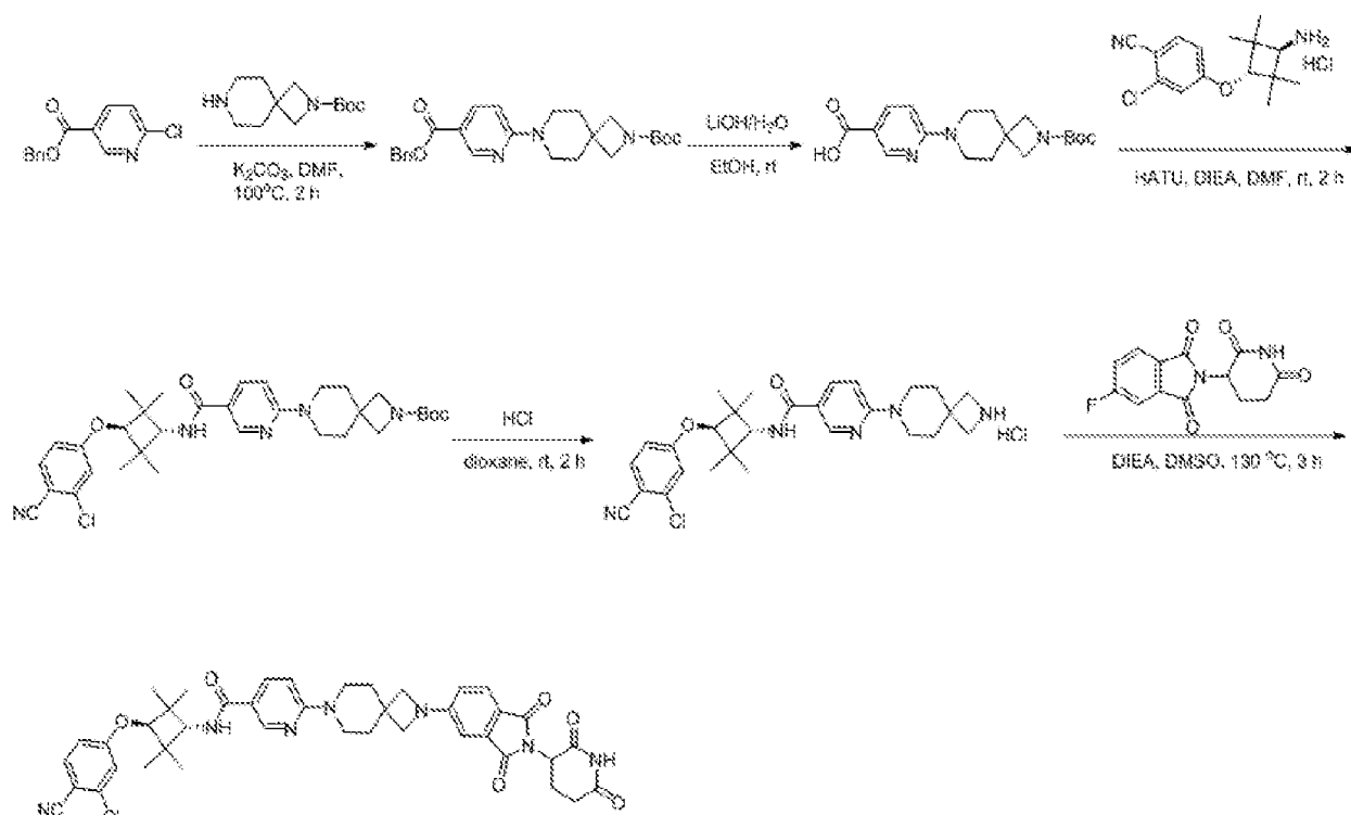
General Scheme 44:
