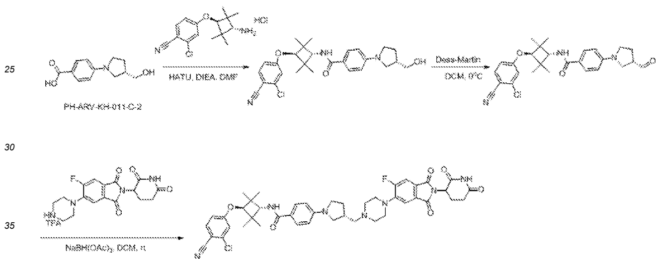
General Scheme 46:
