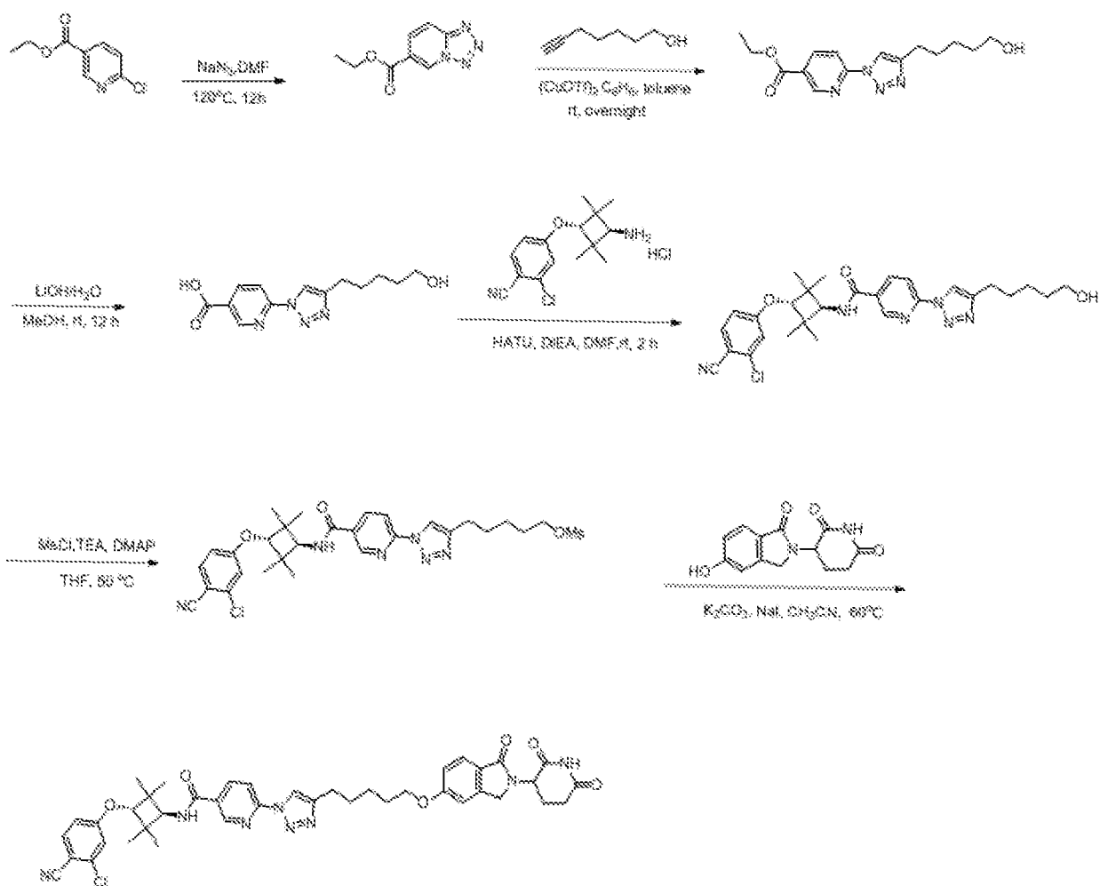
General Scheme 49:
