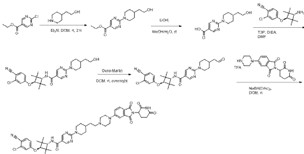
General Scheme 32:
