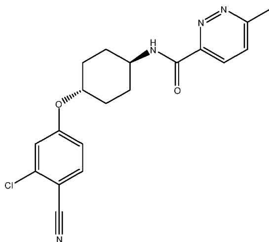
ABM-40: N-((1r,4r)-4-(3-chloro-4-cyanophenoxy)cyclohexyl)-6-methylpyridazine-3-carboxamide
