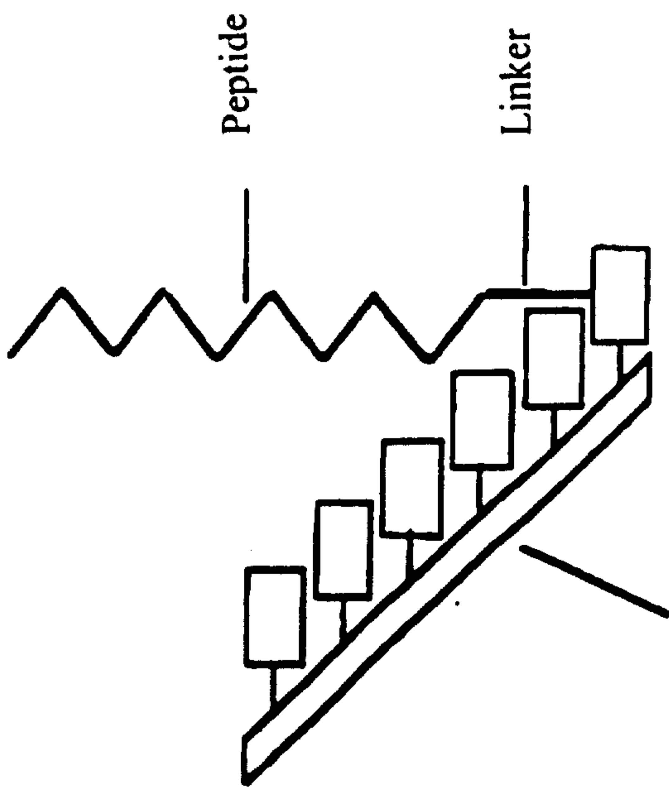
Oligomer from pairing system
