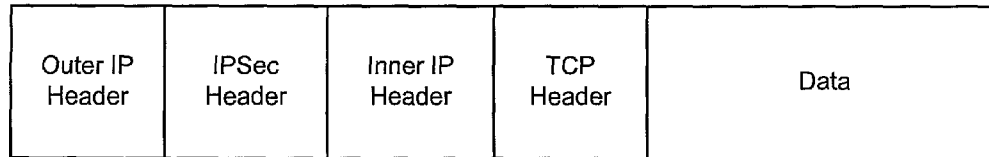
FIG. 7 (Prior Art)
