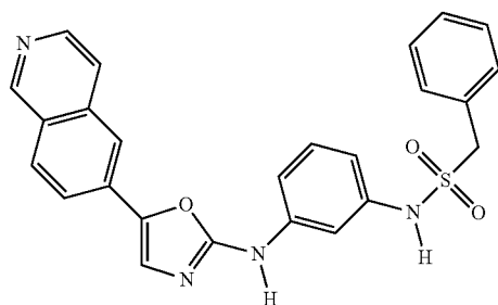
N-(3-((5-(isoquinolin-6-yl)oxazol-2-yl)amino)phenyl)-1-phenylmethanesulfonamide
