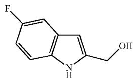
Compound 46: (5-fluoro-1H-indol-2-yl)methanol
