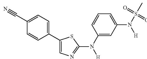
Compound 58: N-(3-((5-(4-cyanophenyl)thiazol-2-yl)amino)phenyl)methanesulfonamide
