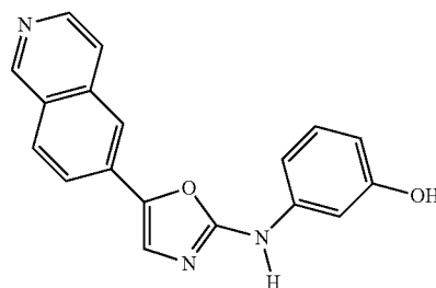
3-((5-(isoquinolin-6-yl)oxazol-2-yl)amino)phenol
