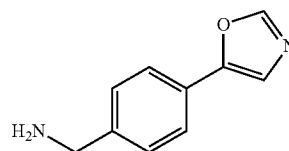
Compound 10: (4-(oxazol-5-yl)phenyl)methanamine
