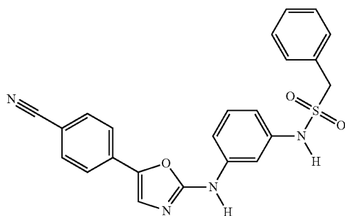
Compound 5: N-(3-((5-(4-cyanophenyl)oxazol-2-yl)amino)phenyl)-1-phenylmethanesulfonamide
