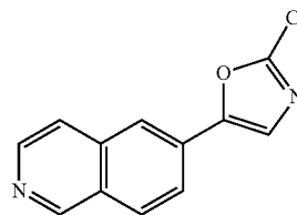
Compound 14: 2-chloro-5-(isoquinolin-6-yl)oxazole
