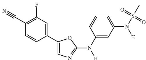
Compound 40: N-(3-((5-(4-cyano-3-fluorophenyl)oxazol-2-yl)amino)phenyl)methanesulfonamide
