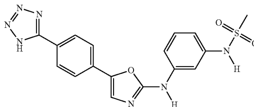
Compound 41: N-(3-((5-(4-(1H-tetrazol-5-yl)phenyl)oxazol-2-yl)amino)phenyl)methanesulfonamide
