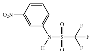
Compound 42: 1,1,1-trifluoro-N-(3-nitrophenyl)methanesulfonamide
