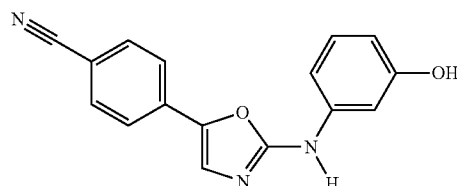
4-(2-((3-hydroxyphenyl)amino)oxazol-5-yl)benzonitrile
