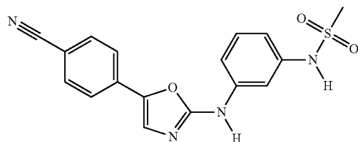
Compound 7: N-(3-((5-(4-cyanophenyl)oxazol-2-yl)amino)phenyl)methanesulfonamide
