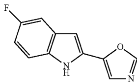
Compound 48: 5-(5-fluoro-1H-indol-2-yl)oxazole
