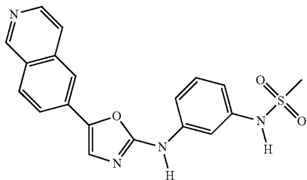
Compound 59: N-(3-((5-(isoquinolin-6-yl)oxazol-2-yl)amino)phenyl)methanesulfonamide
