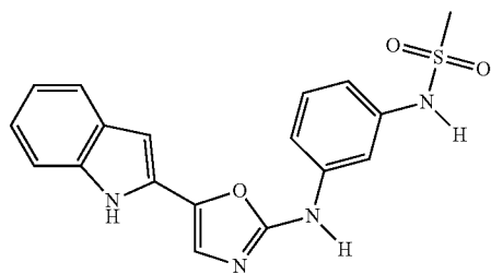
Compound 25: N-(3-((5-(1H-indol-2-yl)oxazol-2-yl)amino)phenyl)methanesulfonamide
