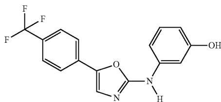
Compound 32: 3-((5-(4-(trifluoromethyl)phenyl)oxazol-2-yl)amino)phenol
