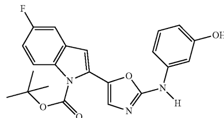
tert-butyl 5-fluoro-2-(2-((3-hydroxyphenyl)amino)oxazol-5-yl)-1H-indole-1-carboxylate
