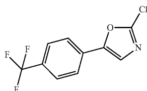
Compound 31: 2-chloro-5-(4-(trifluoromethyl)phenyl)oxazole
