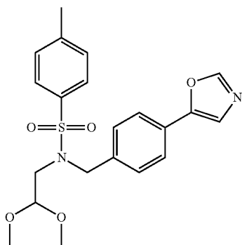
Compound 12: N-(2,2-dimethoxyethyl)-4-methyl-N-(4-(oxazol-5-yl)benzyl)benzenesulfonamide
