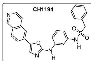
N -(3-((5-(isoquinolin-6-yl)oxazol-2-yl)amino)phenyl)-1-phenylmethanesulfonamide
