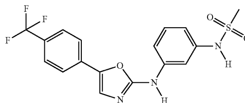
Compound 33: N-(3-((5-(4-(trifluoromethyl)phenyl)oxazol-2-yl)amino)phenyl)methanesulfonamide
