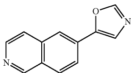
Compound 13: 5-(isoquinolin-6-yl)oxazole
