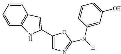
Compound 23: 3-((5-(1H-indol-2-yl)oxazol-2-yl)amino)phenol
