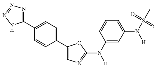
N-(3-((5-(4-(1H-tetrazol-5-yl)phenyl)oxazol-2-yl)amino)phenyl)methanesulfonamide
