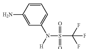
Compound 43: N-(3-aminophenyl)-1,1,1-trifluoromethanesulfonamide
