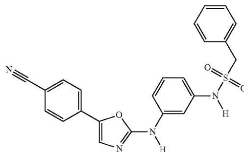
N-(3-((5-(4-cyanophenyl)oxazol-2-yl)amino)phenyl)-1-phenylmethanesulfonamide
