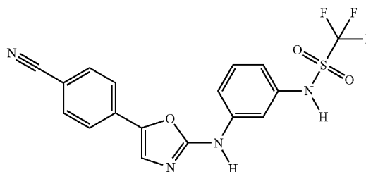
Compound 44: N-(3-((5-(4-cyanophenyl)oxazol-2-yl)amino)phenyl)-1,1,1-trifluoromethanesulfonamide
