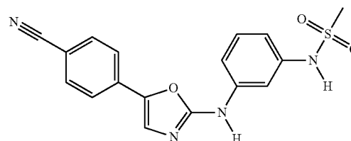
N-(3-((5-(4-cyanophenyl)oxazol-2-yl)amino)phenyl)methanesulfonamide
