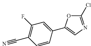
Compound 39: 4-(2-chlorooxazol-5-yl)-2-fluorobenzonitrile
