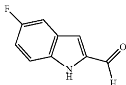
Compound 47: 5-fluoro-1H-indole-2-carbaldehyde
