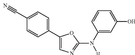
Compound 9: 4-(2-((3-hydroxyphenyl)amino)oxazol-5-yl)benzonitrile
