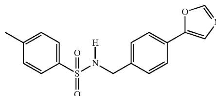
Compound 11: 4-methyl-N-(4-(oxazol-5-yl)benzyl)benzenesulfonamide
