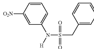
Compound 3:
