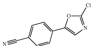
Compound 2: 4-(2-chlorooxazol-5-yl)benzonitrile
