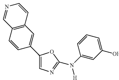
Compound 15: 3-((5-(isoquinolin-6-yl)oxazol-2-yl)amino)phenol
