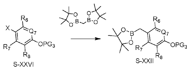
Scheme 6b
