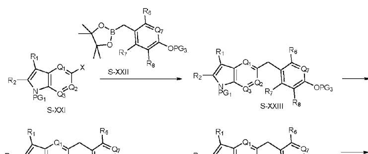
Scheme 6a
