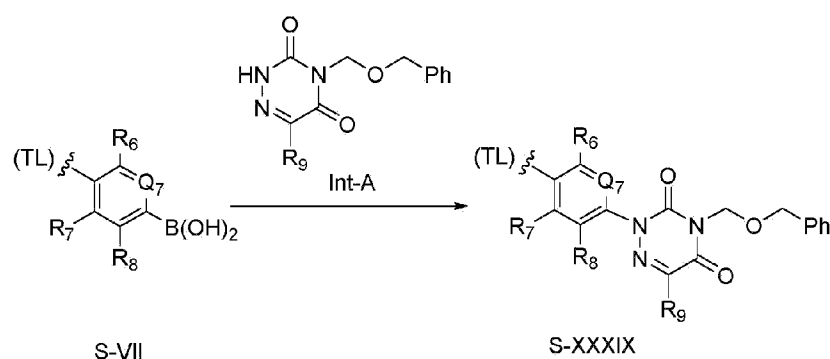
Scheme 12
