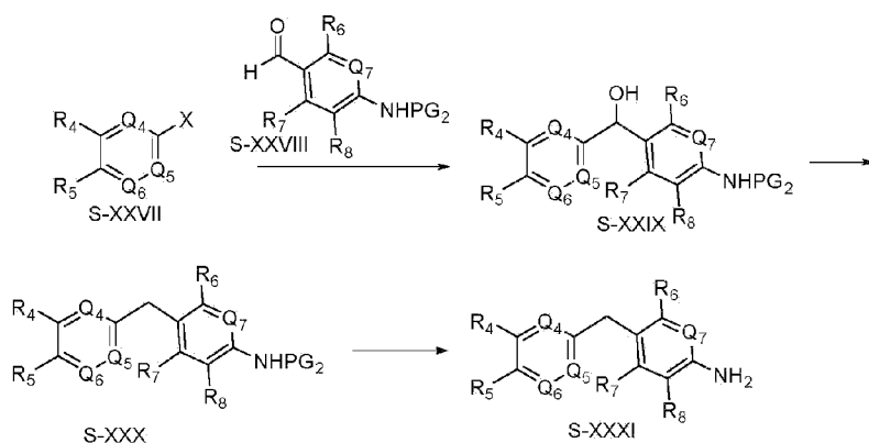
Scheme 7
