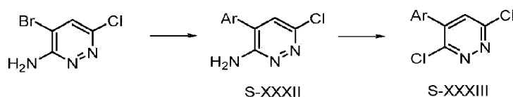
Scheme 9
