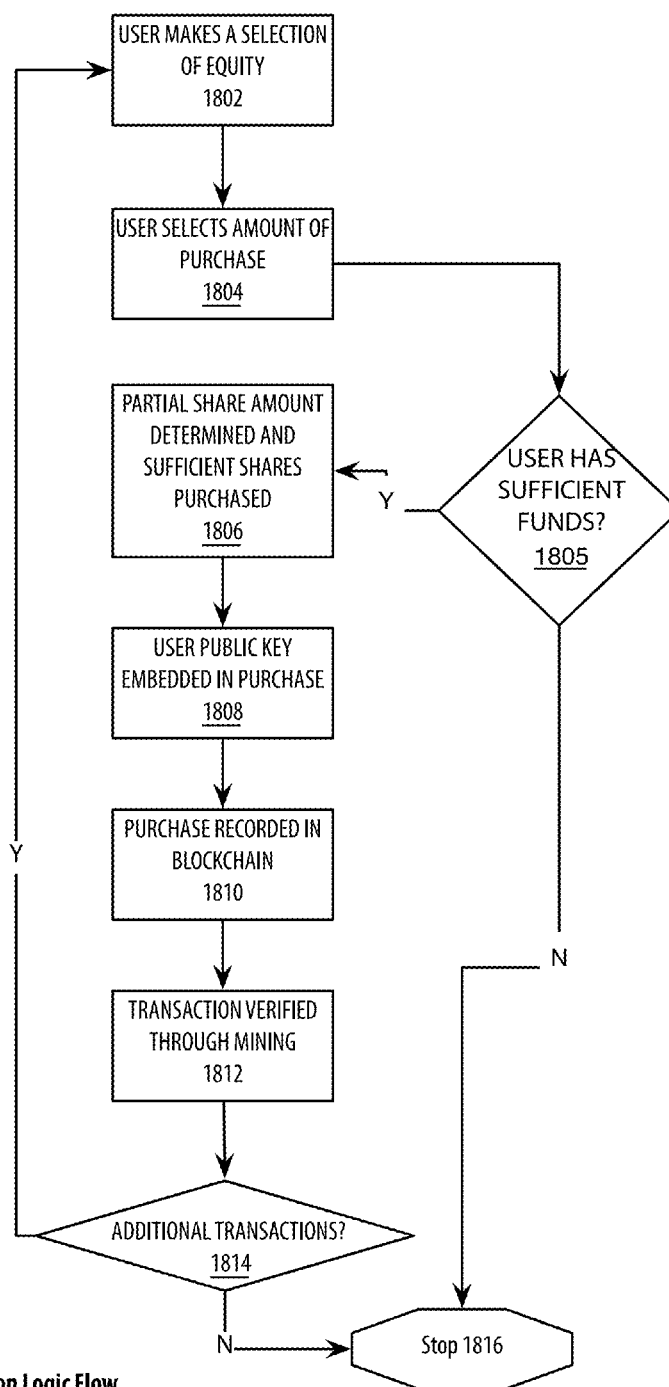
Fig. 18: SOCOACT—Transaction Logic Flow
