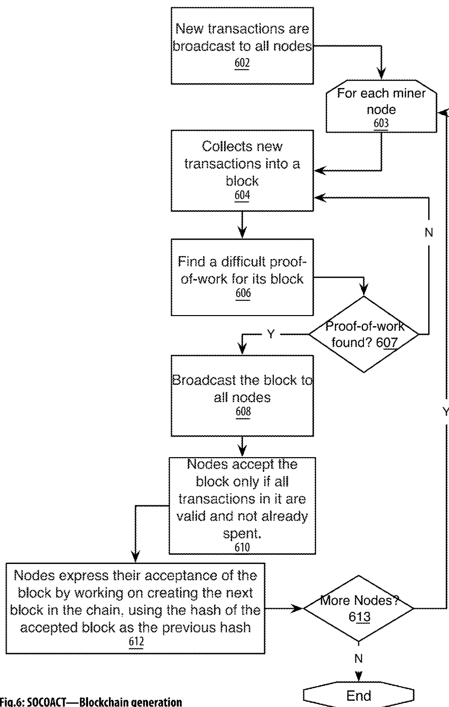
Fig.6: SOCOACT—Blockchain generation
