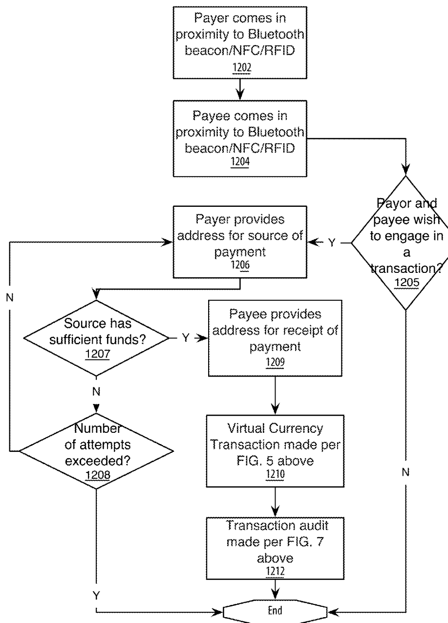
Fig.12: SOCOACT—Verified BET transactions
