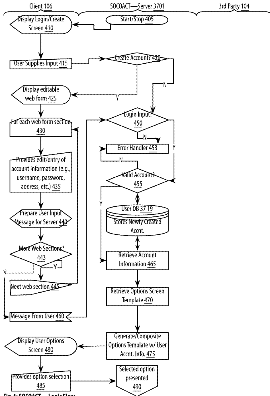
Fig.4: SOCOACT—Logic Flow
