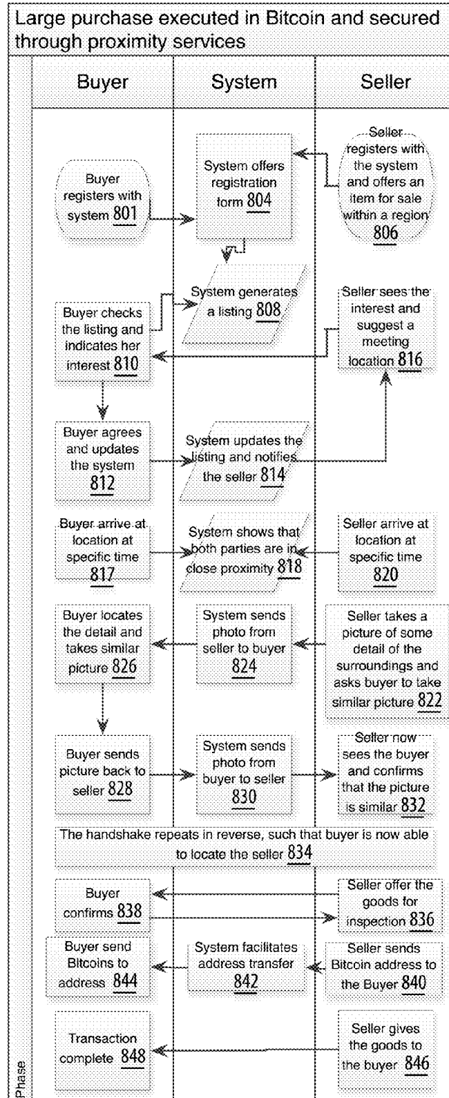
Fig.8: SOCOACT—Transactions
