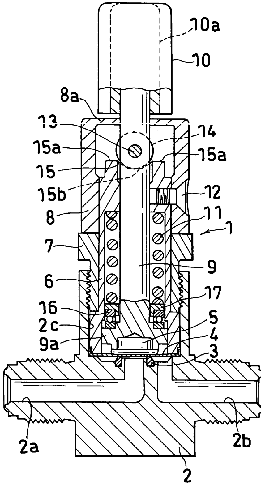
Fig. 4 (PRIOR ART)
