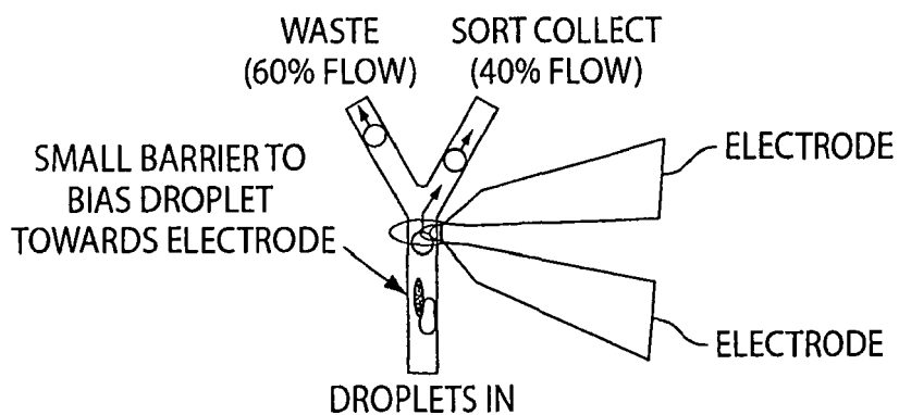
BIASED DESIGN
