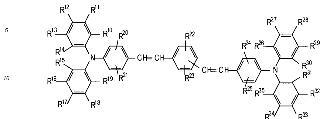
General Formula (4)
