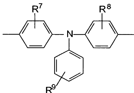
Structural Formula (3-1)
