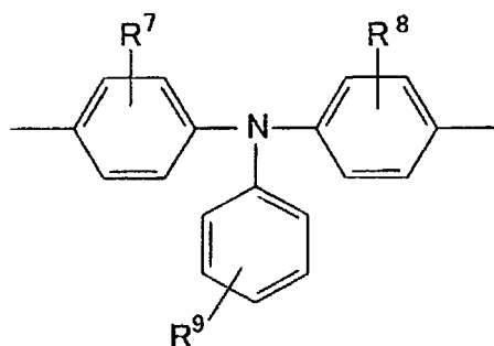
Structural Formula (3-1)
