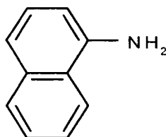
Structural Formula (2)
