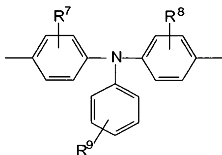
Structural Formula (3-1)
