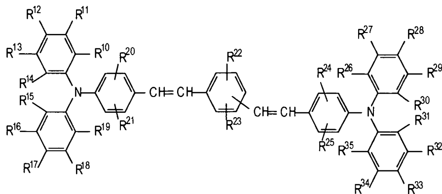
General Formula (4)
