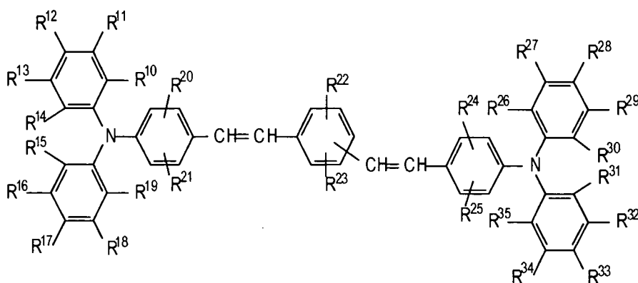
General Formula (4)
