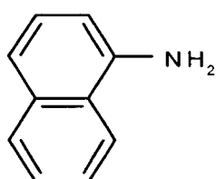
Structural Formula (2)
