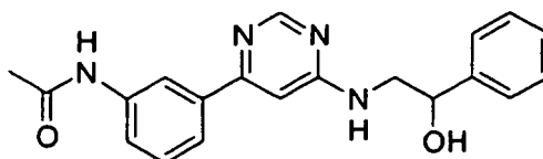
Example 243: 1-Phenyl-2-(6-phenyl-pyrimidin-4-ylamino)-ethanol.
