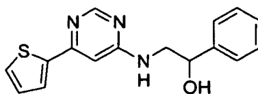
Example 245: 1-Phenyl-2-(6-thiophen-3-yl-pyrimidin-4-ylamino)-ethanol.
