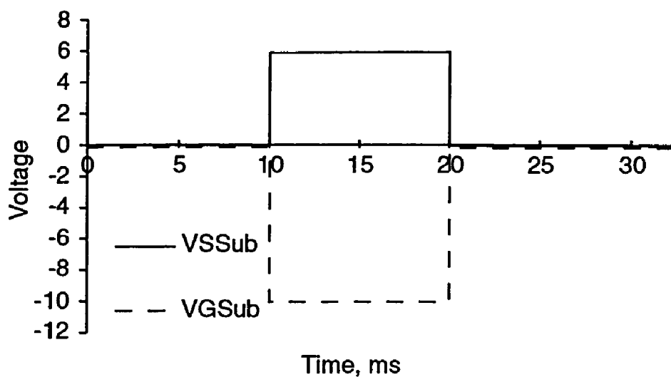
Fig. 3 Prior Art
