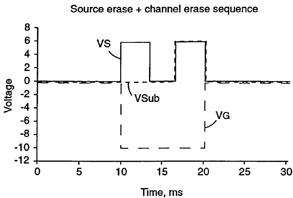
Fig. 5 Prior Art
