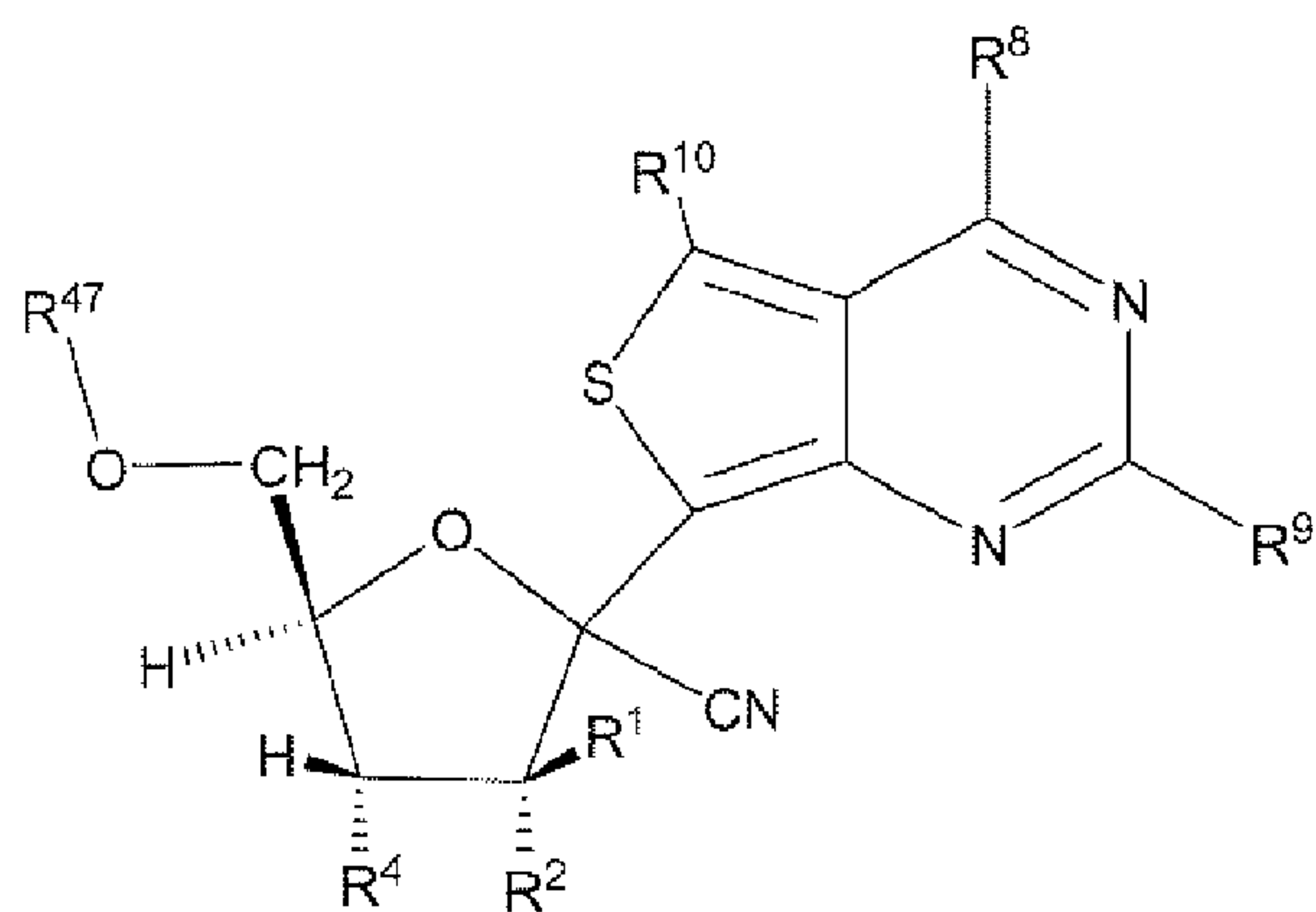
Formula IVb
