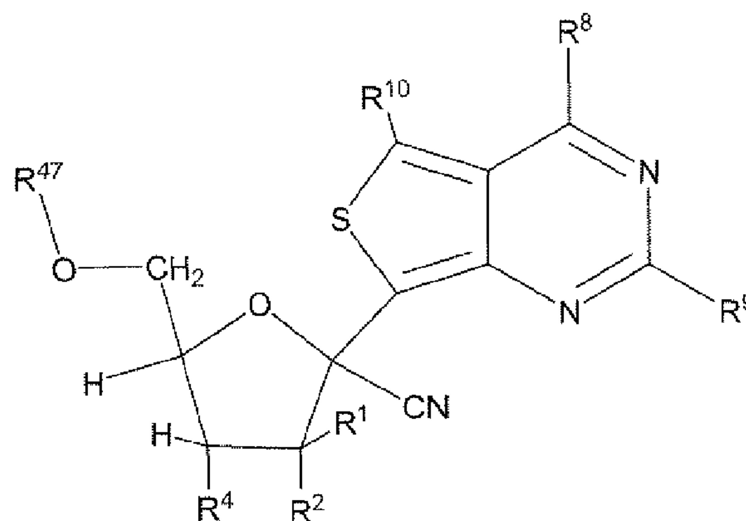
Formula IV
