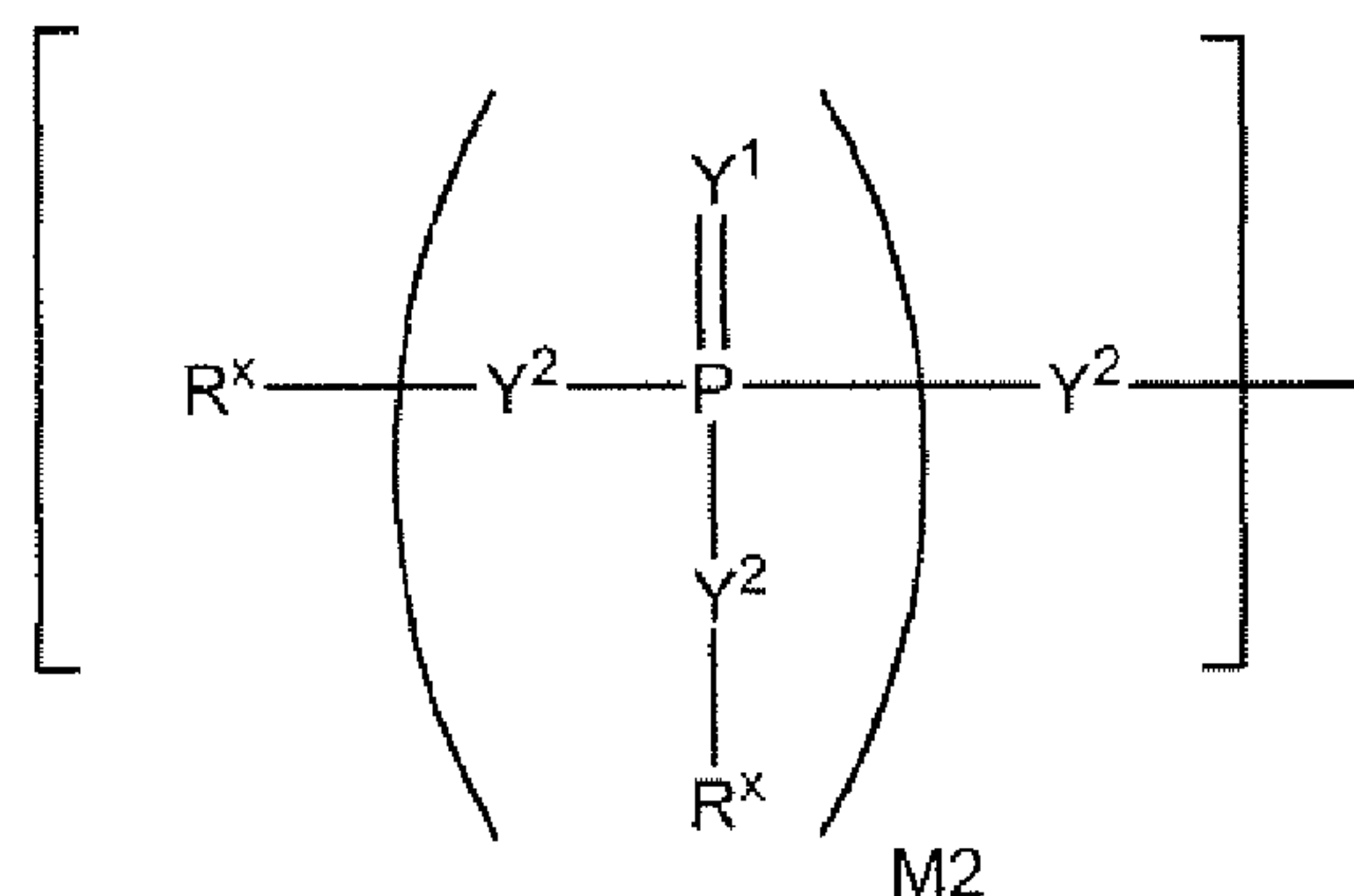
Formula Ia
