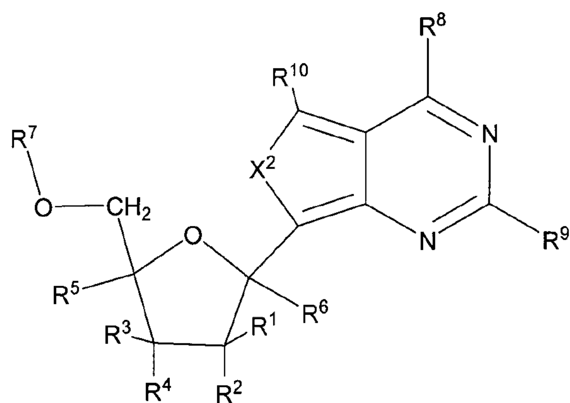
Formula I
