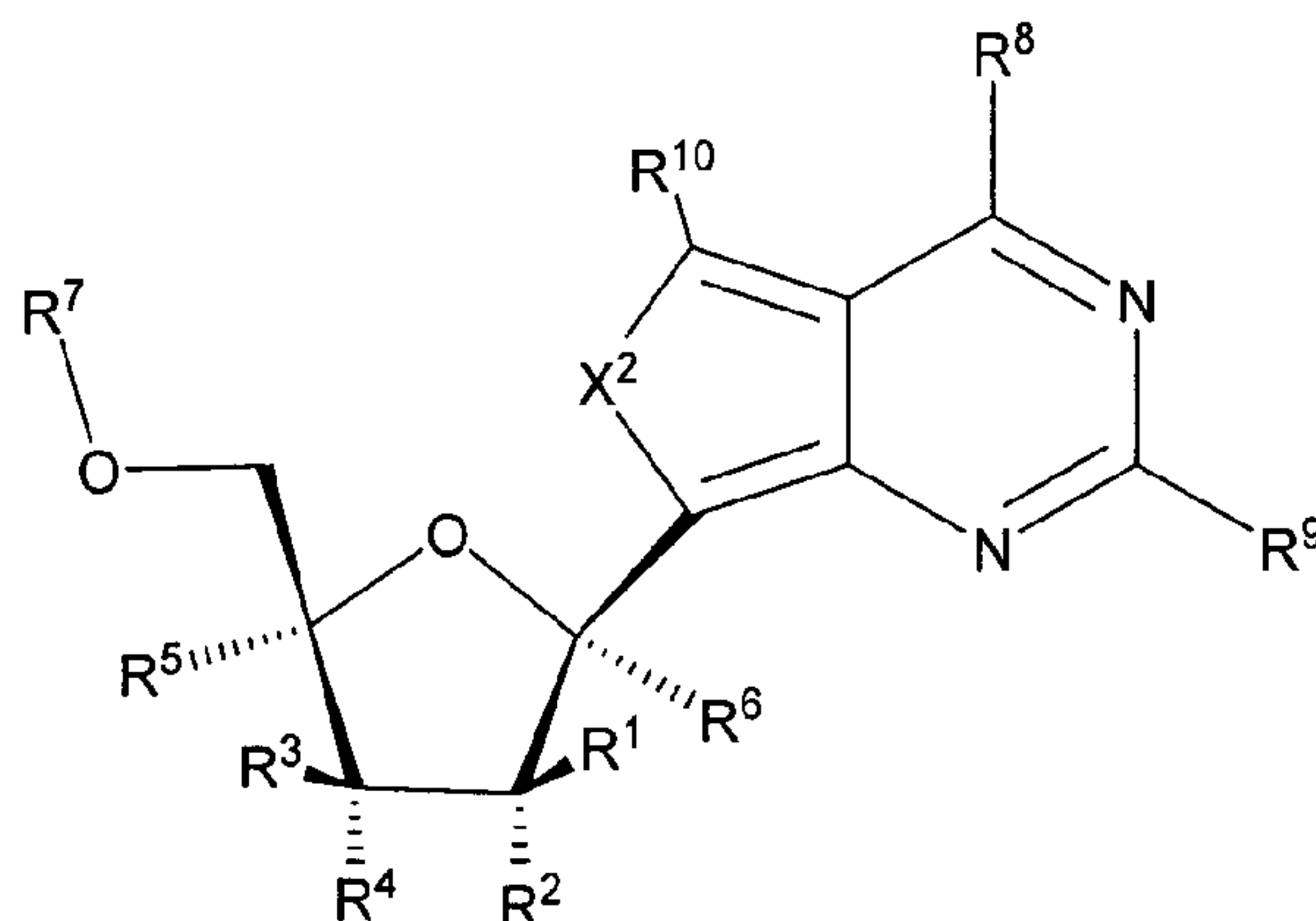
Formula II.
