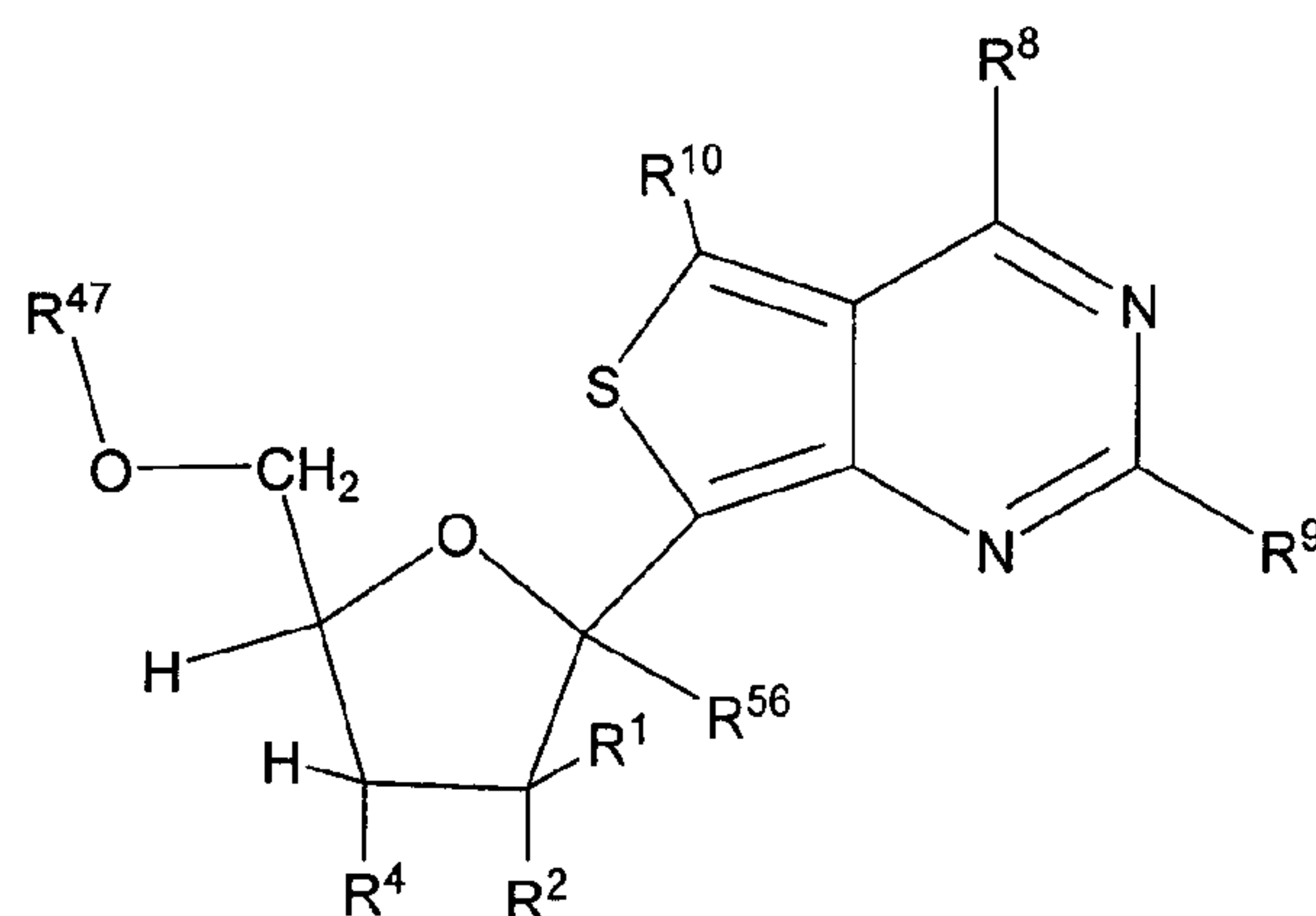
Formula V
