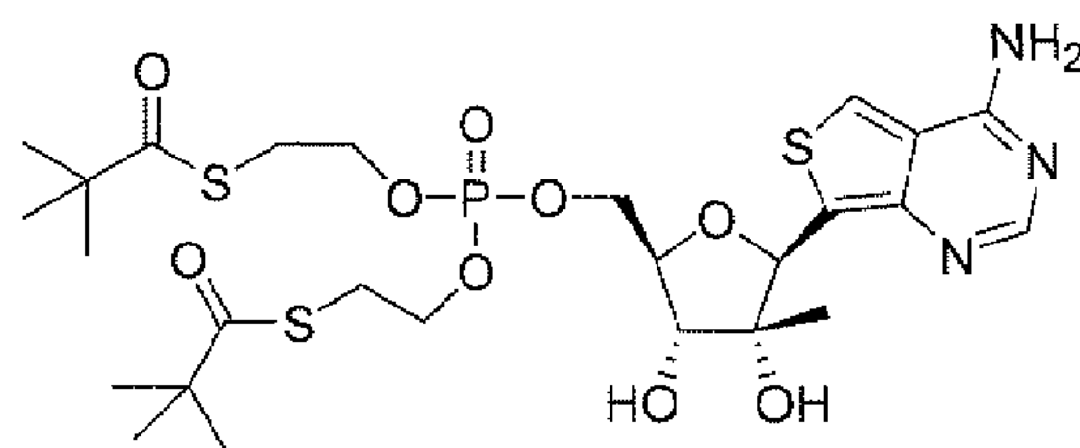
Compound 2
