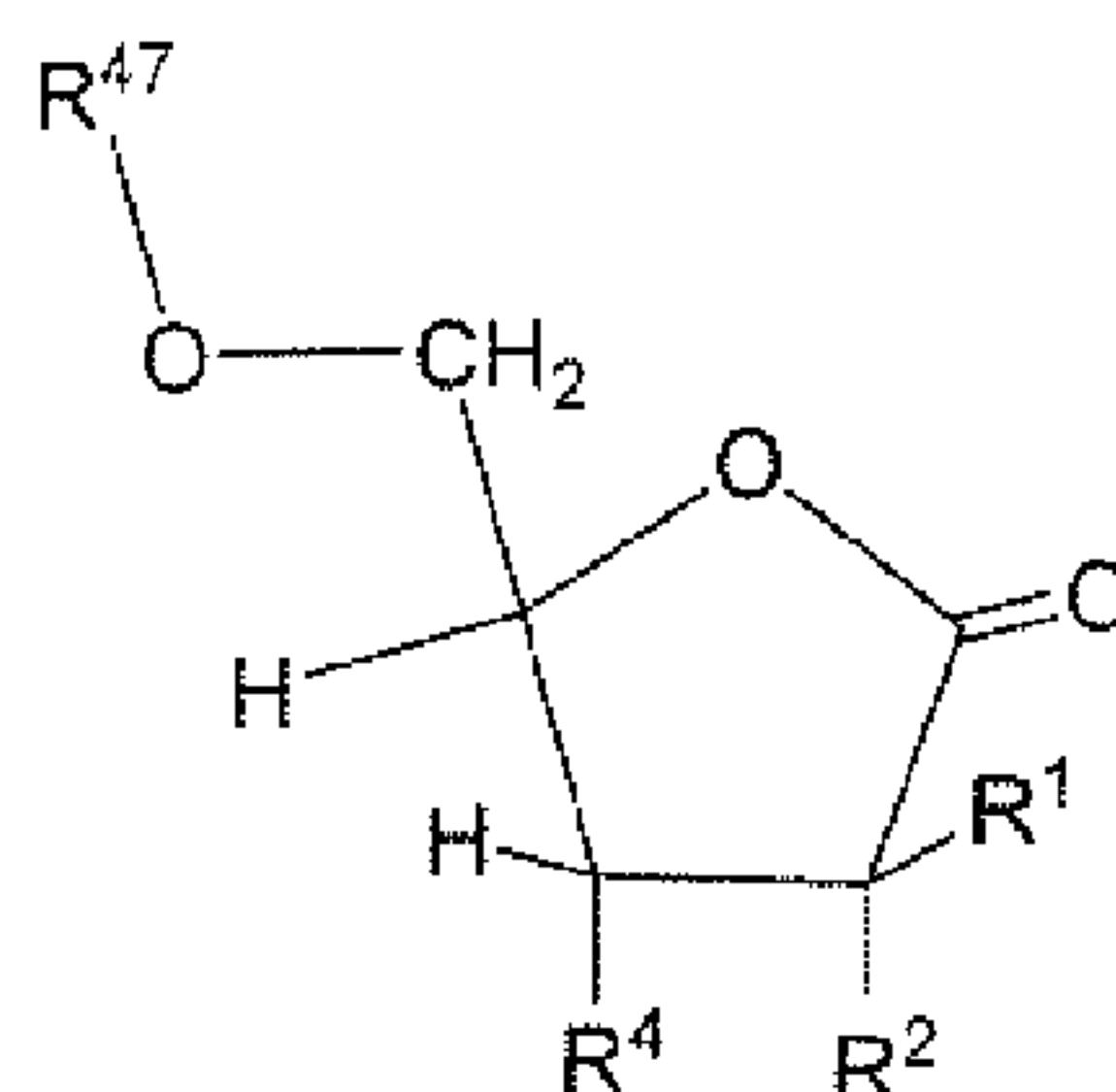
Formula VI
