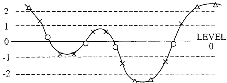
WAVEFORM EQUALIZING SIGNAL HAVING CROSS-TALK
