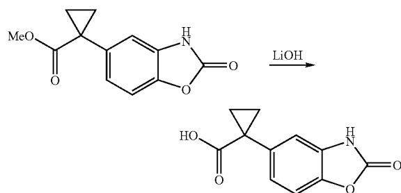
1-(2-Oxo-2,3-dihydrobenzo[d]oxazol-5-yl)cyclopropanecarboxylic acid
