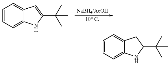
2-tert-Butylindoline
