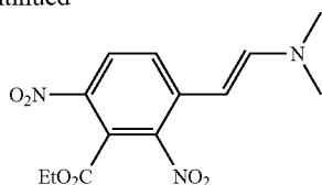
(E)-Ethyl 3-(2-(dimethylamino)vinyl)-2,6-dinitrobenzoate
