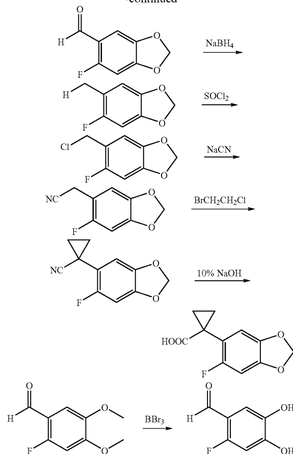
2-Fluoro-4,5-dihydroxy-benzaldehyde
