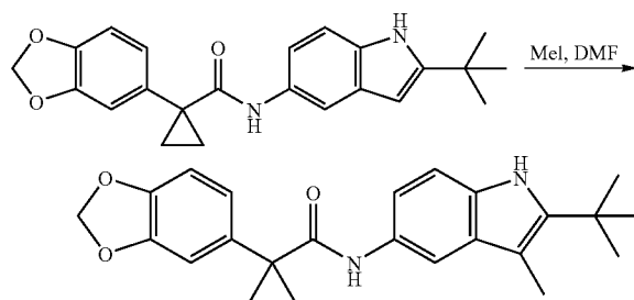
1-(Benzo[d][1,3]dioxol-5-yl)-N-(2-tert-butyl-3-methyl-1H-indol-5-yl)cyclopropanecarboxamide
