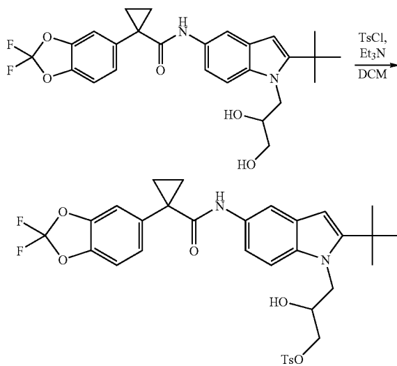
3-(2-tert-Butyl-5-(1-(2,2-difluorobenzo[d][1,3]dioxol-5-yl)cyclopropanecarbox-amido)-1H-indol-1-yl)-2-hydroxypropyl-4-methylbenzenesulfonate
