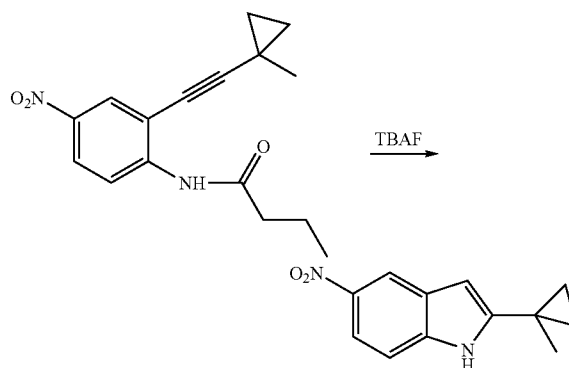
2-(1-Methylcyclopropyl)-5-nitro-1H-indole
