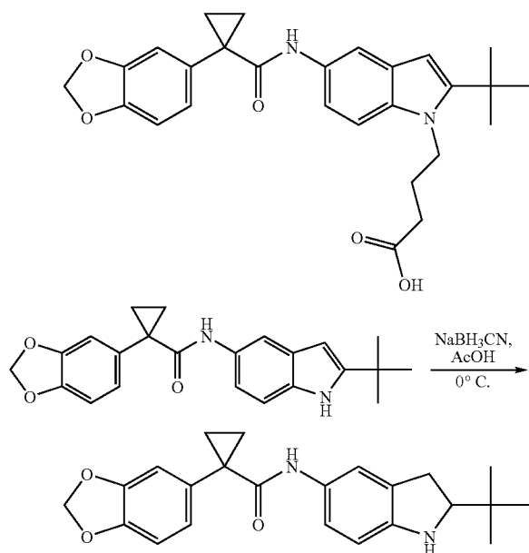
1-(Benzo[d][1,3]dioxol-5-yl)-N-(2-tert-butylindolin-5-yl)cyclopropanecarboxamide
