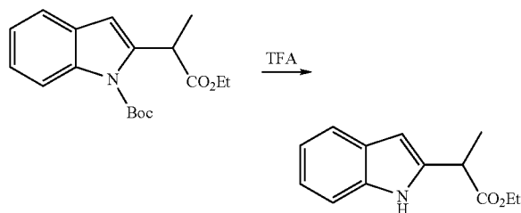
Ethyl 2-(1H-indol-2-yl)propanoate
