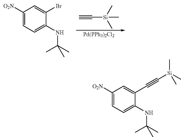
tert-Butyl-(4-nitro-2-trimethylsilanylethynyl-phenyl)-amine
