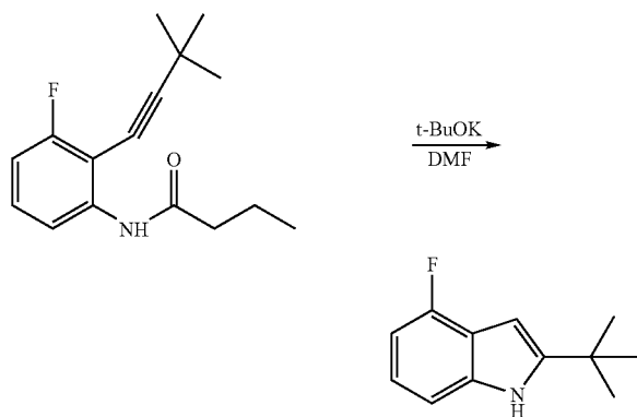
2-tert-Butyl-4-fluoro-1H-indole
