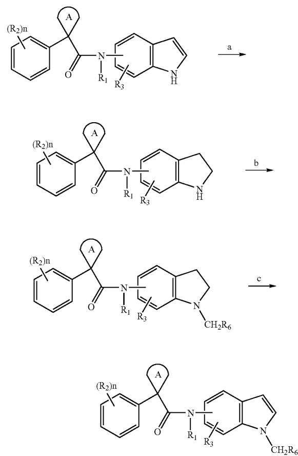
Scheme 35
