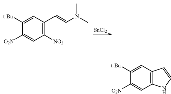
5-tert-Butyl-1H-indol-6-amine
