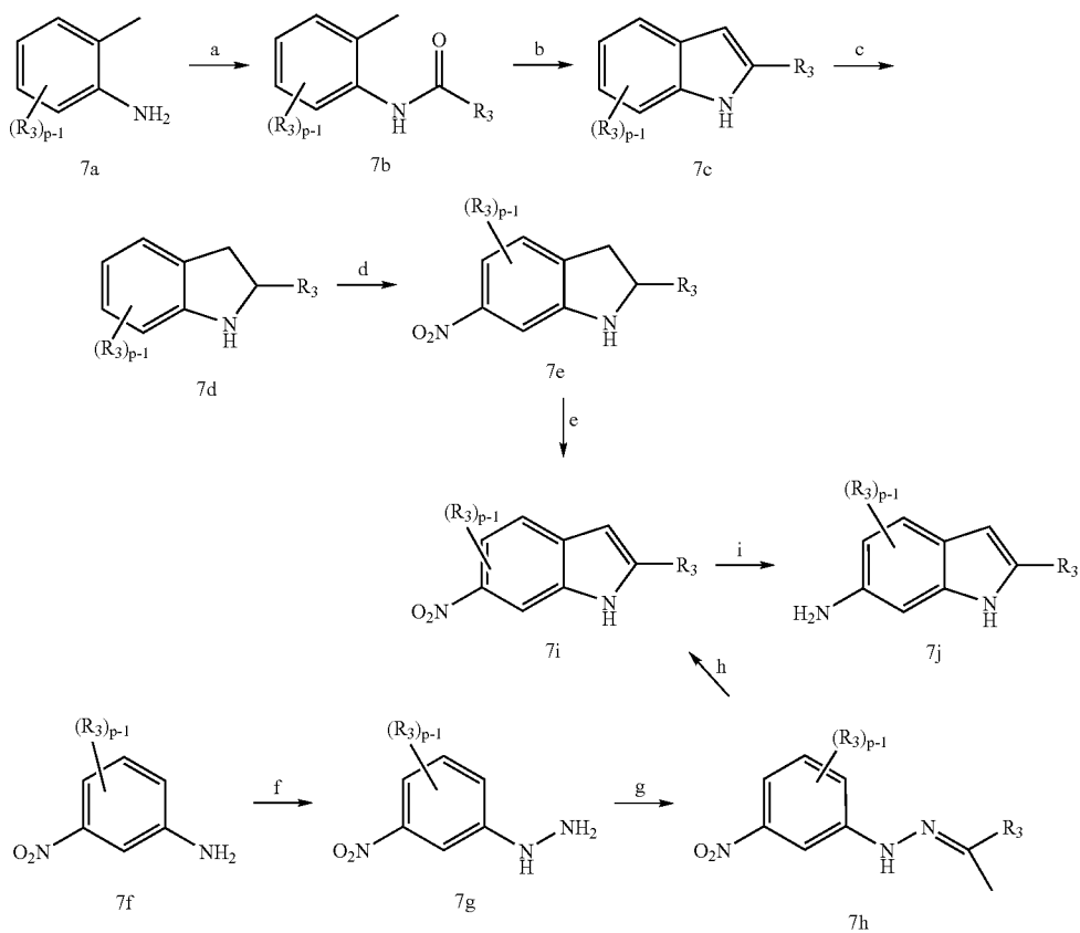
Scheme 7
