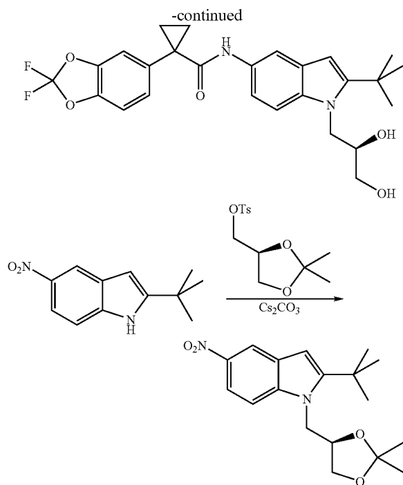
(R)-2-tert-Butyl-1-((2,2-dimethyl-1,3-dioxolan-4-yl)methyl)-5-nitro-1H-indole
