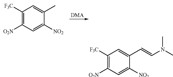
(E)-2-(2,4-Dinitro-5-(trifluoromethyl)-phenyl)-N,N-dimethylethenamine
