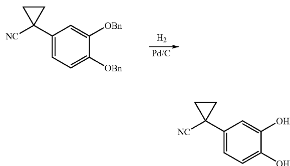
1-(3,4-Dihydroxy-phenyl)-cyclopropanecarbonitrile
