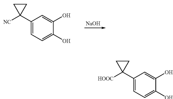
1-(3,4-Dihydroxy-phenyl)-cyclopropanecarboxylic acid
