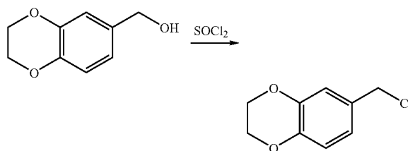
6-Chloromethyl-2,3-dihydro-benzo[1,4]dioxine
