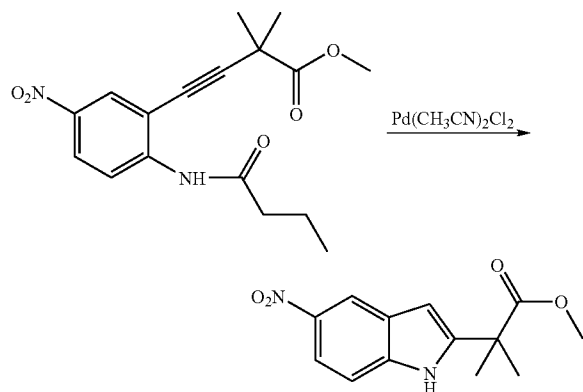
Methyl 2-methyl-2-(5-nitro-1H-indol-2-yl)propanoate
