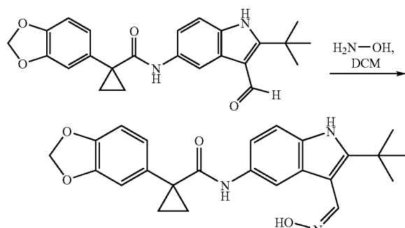
(Z)-1-(Benzo[d][1,3]dioxol-5-yl)-N-(2-tert-butyl-3-((hydroxyimino)methyl)-1H-indol-5-yl)cyclopropanecarboxamide
