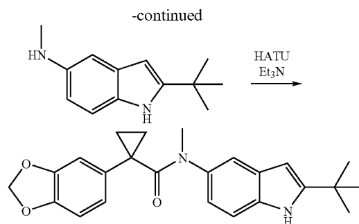
1-(Benzo[d][1,3]dioxol-5-yl)-N-(2-tert-butyl-1H-indol-5-yl)-N-methylcyclopropanecarboxamide
