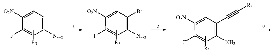
Scheme 18
