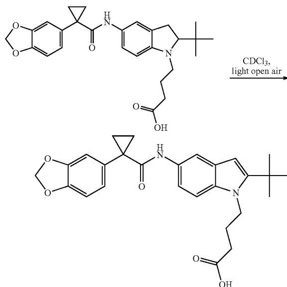
4-(5-(1-(Benzo[d][1,3]dioxol-5-yl)cyclopropanecarboxamido)-2-tert-butyl-1H-indol-1-yl)butanoic acid
