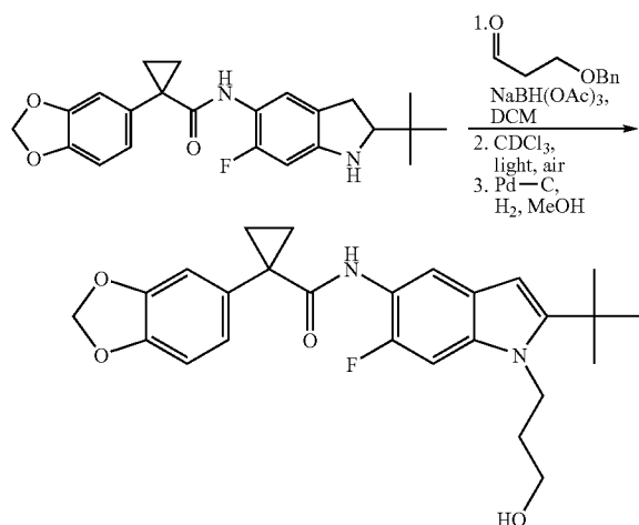
1-(Benzo[d][1,3]dioxol-5-yl)-N-(2-tert-butyl-6-fluoro-1-(3-hydroxypropyl)-1H-indol-5-yl)cyclopropanecarboxamide
