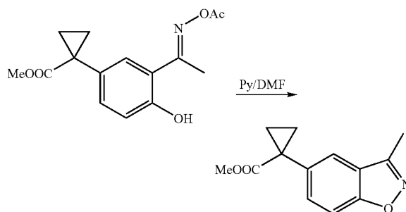
Methyl 1-(3-methylbenzo[d]isoxazol-5-yl)cyclopropanecarboxylate
