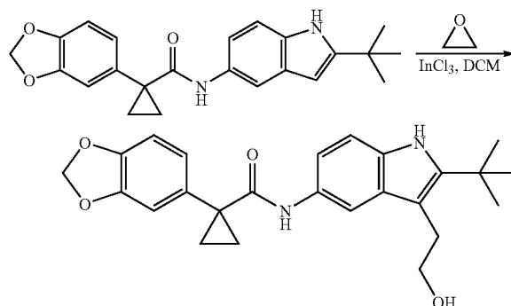
1-(Benzo[d][1,3]dioxol-5-yl)-N-(2-tert-butyl-3-(2-hydroxyethyl)-1H-indol-5-yl)cyclopropanecarboxamide
