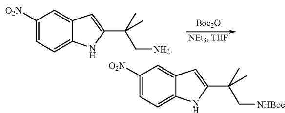
tert-Butyl 2-methyl-2-(5-nitro-1H-indol-2-yl)propylcarbamate
