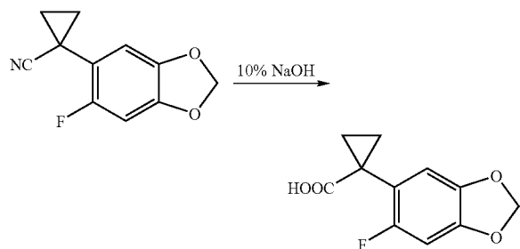
1-(6-Fluoro-benzo[1,3]dioxol-5-yl)-cyclopropanecarboxylic acid
