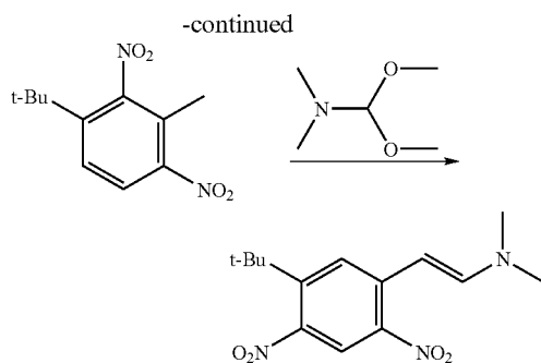
(E)-2-(5-tert-Butyl-2,4-dinitrophenyl)- N,N-dimethylethanamine
