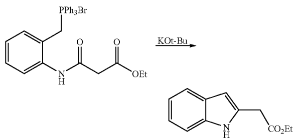
Ethyl 2-(1H-indol-2-yl)acetate
