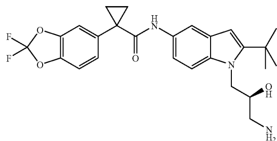
(S)—N-(1-(3-Amino-2-hydroxypropyl)-2-tert-butyl-1H-indol-5-yl)-1-(2,2-difluorobenzo[d][1,3]dioxol-5-yl)cyclopropanecarboxamide
