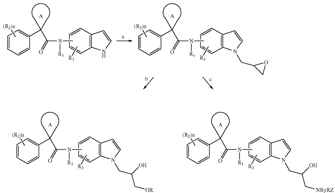
Scheme 39
