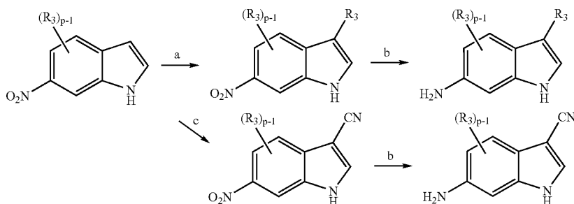
Scheme 15
