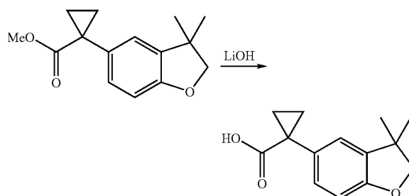
1-(3,3-Dimethyl-2,3-dihydrobenzofuran-5-yl)cyclopropanecarboxylic acid
