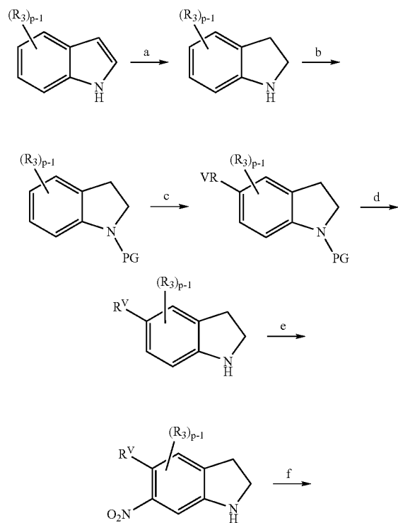
Scheme 13
