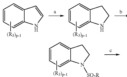
Scheme 14
