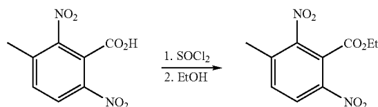
Ethyl 3-methyl-2,6-dinitrobenzoate
