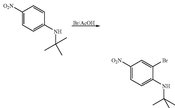
(2-Bromo-4-nitro-phenyl)-tert-butyl-amine
