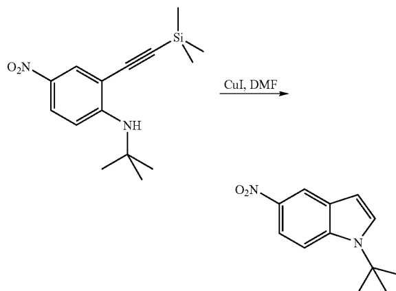
1-tert-Butyl-5-nitro-1H-indole
