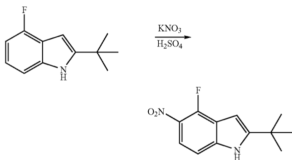
2-tert-Butyl-4-fluoro-5-nitro-1H-indole
