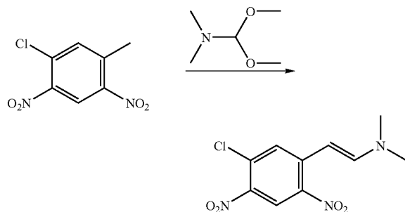
(E)-2-(5-Chloro-2,4-dinitrophenyl)- N,N-dimethylethenamine
