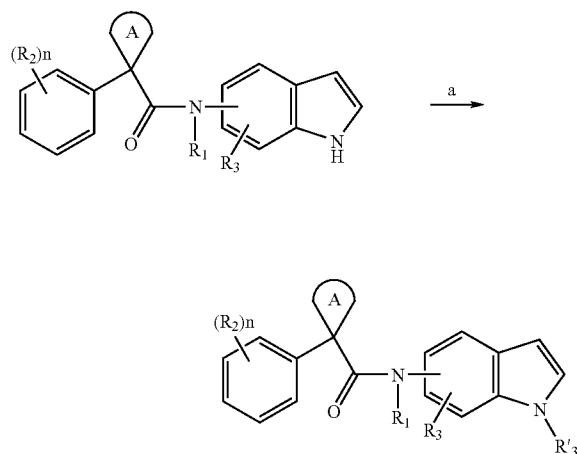
Scheme 36
