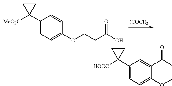
1-(4-Oxochroman-6-yl)cyclopropanecarboxylic acid
