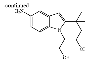
3-[5-Amino-1-(2-hydroxy-ethyl)-1H-indol-2-yl]-3-methyl-butan-1-ol
