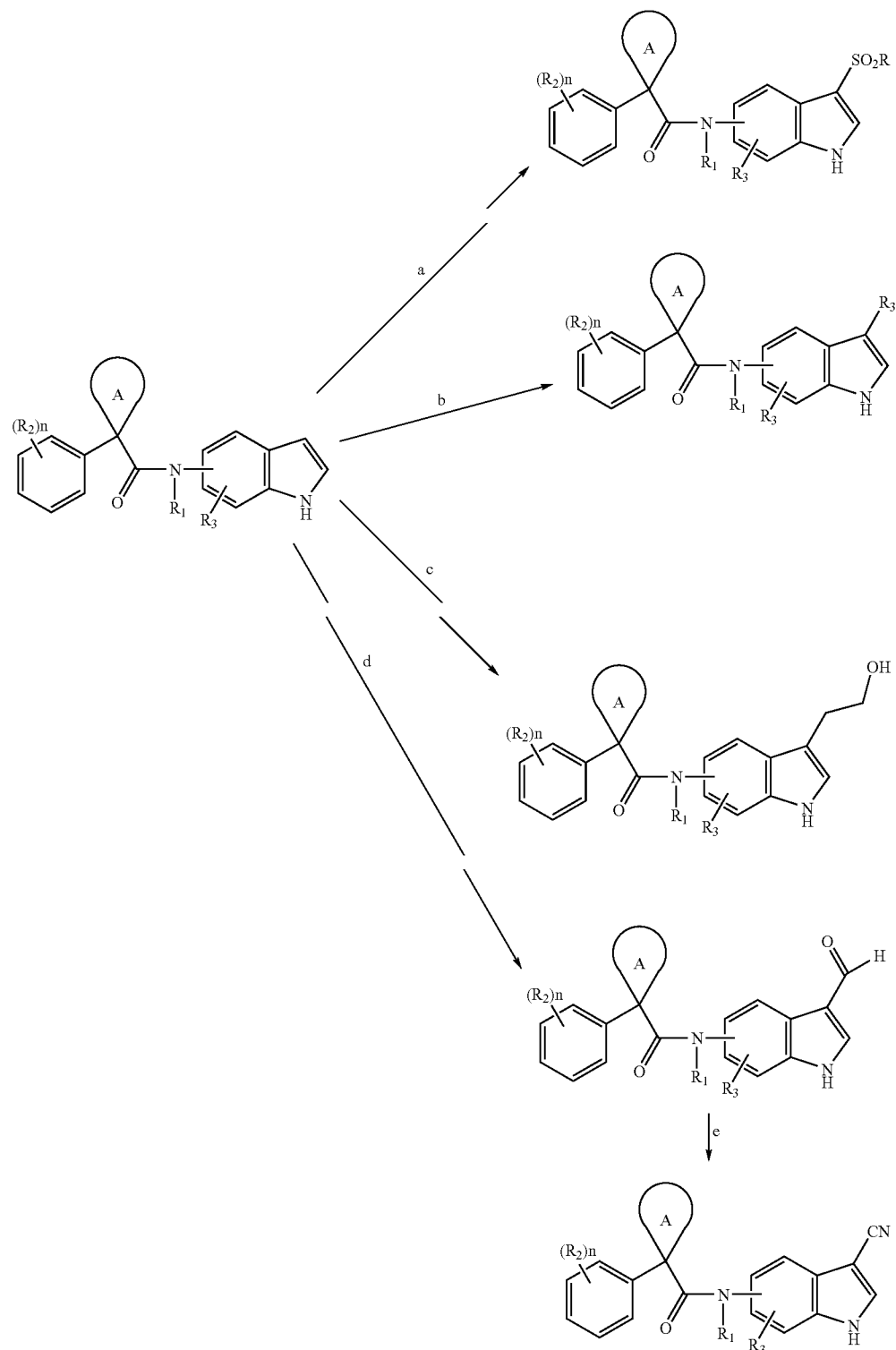
Scheme 38
