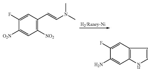
5-Fluoro-1H-indol-6-amine
