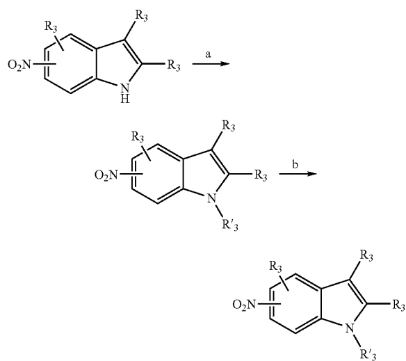
Scheme 16
