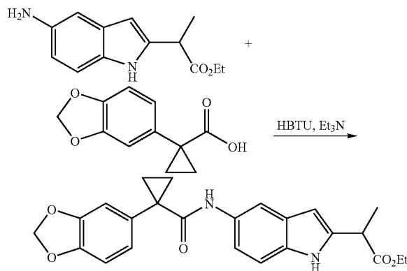
Ethyl 2-(5-(1-(benzo[d][1,3]dioxol-5-yl)cyclopropanecarboxamido)-1H-indol-2-yl)propanoate
