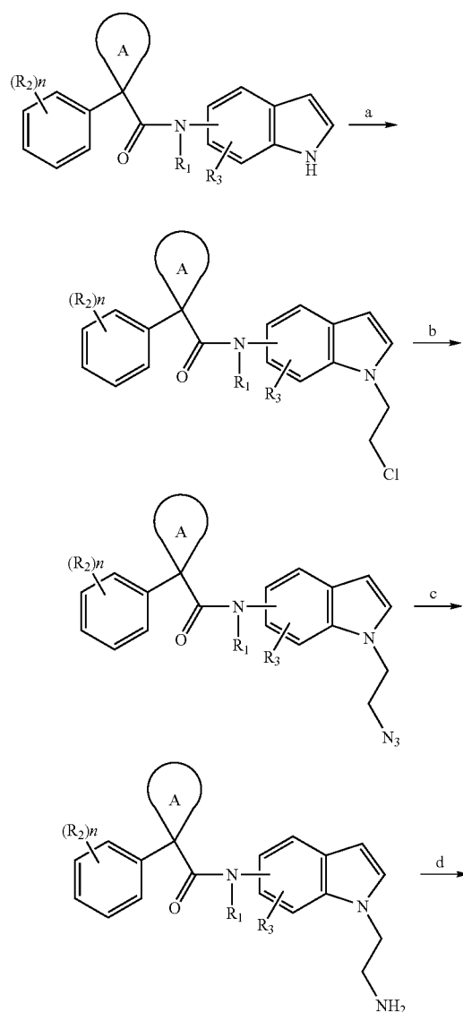
Scheme 41
