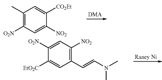
Ethyl 6-amino-1H-indole-5-carboxylate
