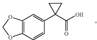
1-(Benzo[d][1,3]dioxol-5-yl)-N-(2-tert-butyl-1H-indol-5-yl)-N-methylcyclopropanecarboxamide
