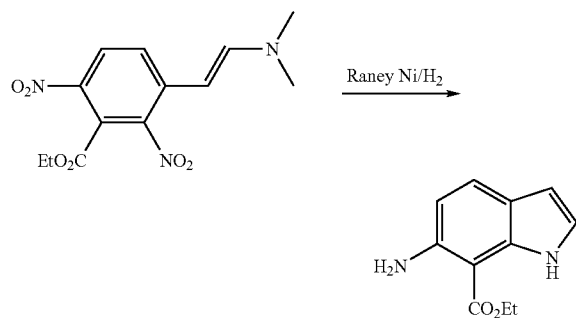
Ethyl 6-amino-1H-indole-7-carboxylate
