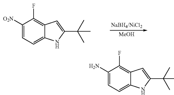
2-tert-Butyl-4-fluoro-1H-indol-5-amine
