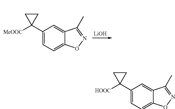
1-(3-Methylbenzo[d]isoxazol-5-yl)cyclopropanecarboxylic acid
