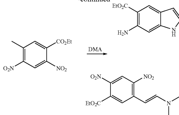
(E)-Ethyl 5-(2-(dimethylamino)vinyl)-2,4-dinitrobenzoate
