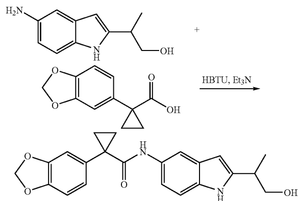
1-(Benzo[d][1,3]dioxol-5-yl)-N-(2-(1-hydroxypropan-2-yl)-1H-indol-5-yl)cyclopropanecarboxamide
