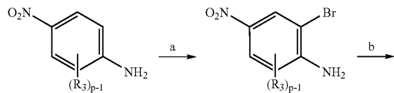
Scheme 17
