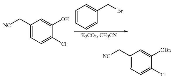
2-(3-(Benzyloxy)-4-chlorophenyl)acetonitrile
