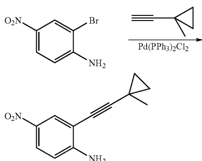
2-((1-Methylcyclopropyl)ethynyl)-4-nitroaniline
