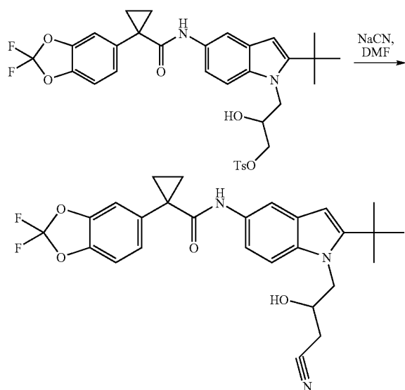
N-(2-tert-Butyl-1-(3-cyano-2-hydroxypropyl)-1H-indol-5-yl)-1-(2,2-difluorobenzo[d][1,3]dioxol-5-yl)cyclopropanecarboxamide
