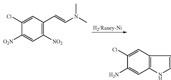
5-Chloro-1H-indol-6-amine
