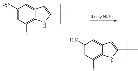
2-tert-Butyl-7-fluoro-1H-indol-5-amine
