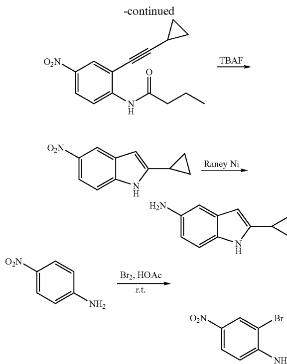
2-Bromo-4-nitroaniline
