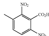
3-Methyl-2,6-dinitrobenzoic acid
