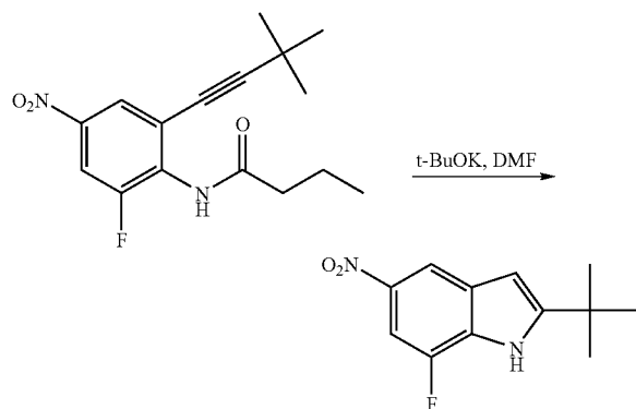
2-tert-Butyl-7-fluoro-5-nitro-1H-indole
