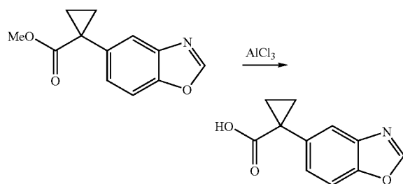
1-(Benzo[d]oxazol-5-yl)cyclopropanecarboxylic acid
