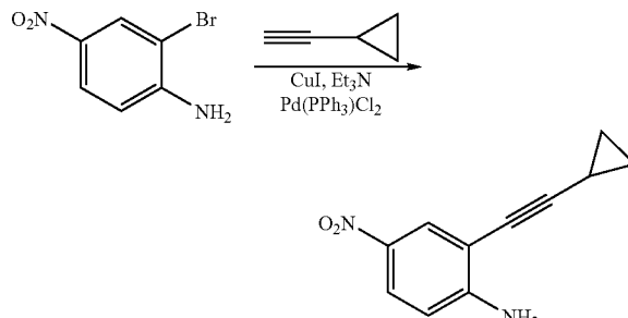
2-(Cyclopropylethynyl)-4-nitroaniline
