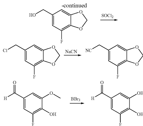
3-Fluoro-4,5-dihydroxy-benzaldehyde
