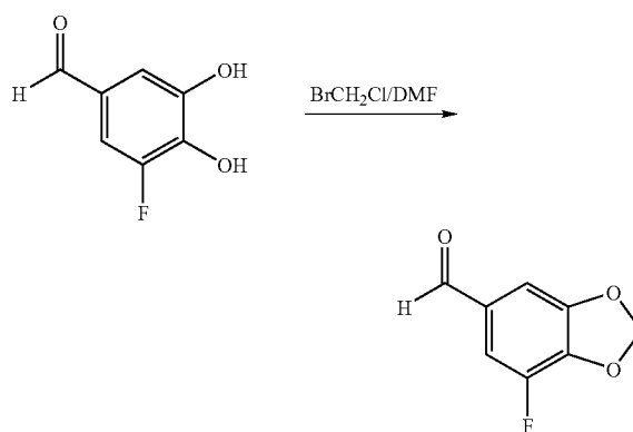
7-Fluoro-benzo[1,3]dioxole-5-carbaldehyde
