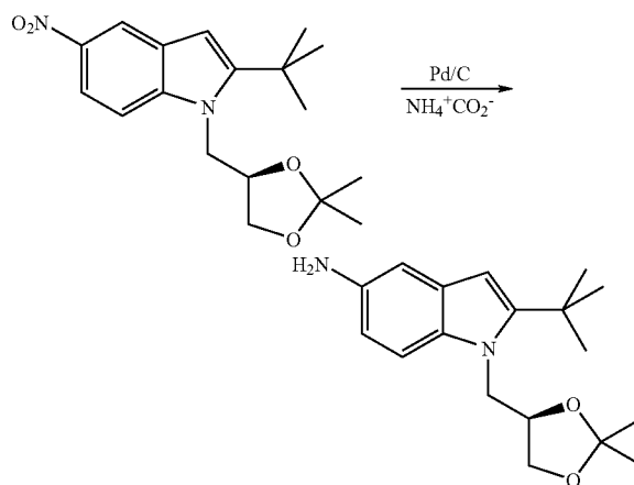
(R)-2-tert-Butyl-1-((2,2-dimethyl-1,3-dioxolan-4-yl)methyl)-5-amine-1H-indole
