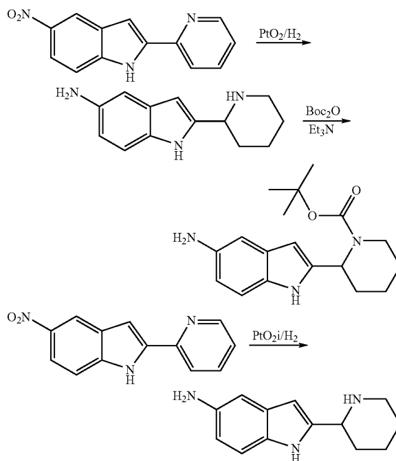
2-(Piperidin-2-yl)-1H-indol-5-amine
