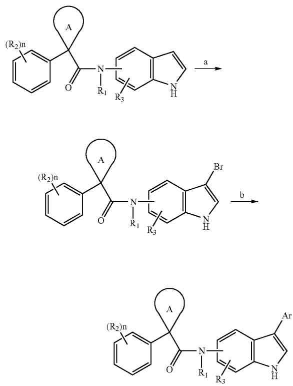
Scheme 37
