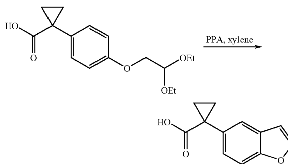
1-Benzofuran-5-yl-cyclopropanecarboxylic acid
