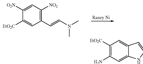
Ethyl 6-amino-1H-indole-5-carboxylate
