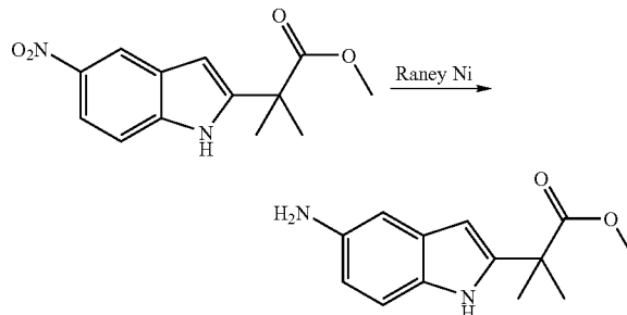
Methyl 2-(5-amino-1H-indol-2-yl)-2-methylpropanoate
