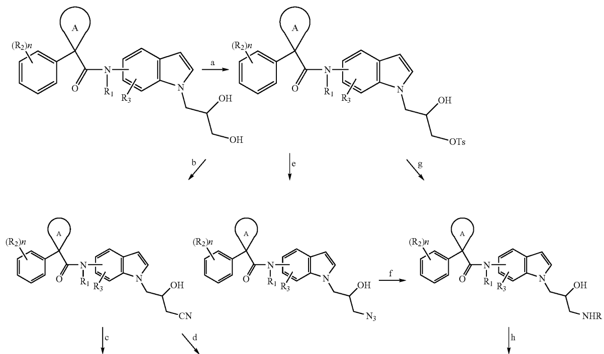
Scheme 40
