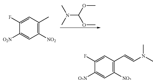
(E)-2-(5-Fluoro-2,4-dinitrophenyl)- N,N-dimethylethenamine
