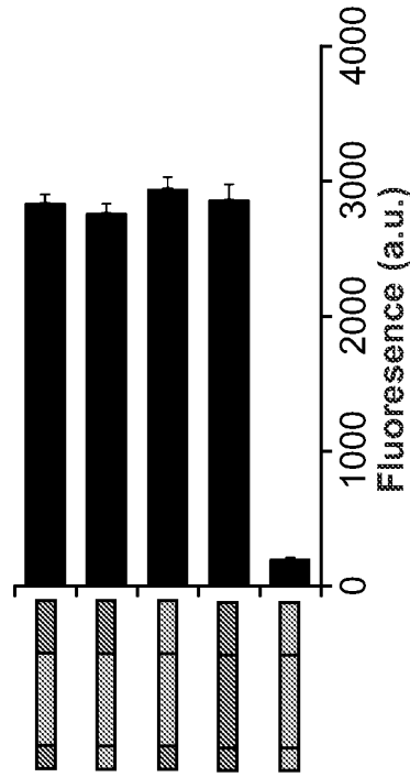
FIG. 10C NM gRNA with NM reporter PAM
