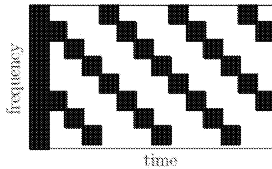
Diagonal pilot structure
