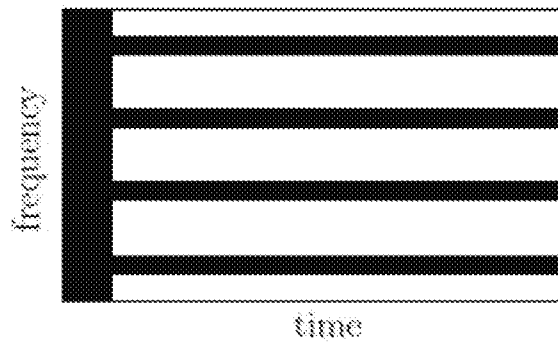
Comb-type in frequency domain
