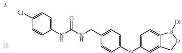
1-(4-Chloro-phenyl)-3-[4-(1-hydroxy-1,3-dihydro-benzo[c][1,2]oxaborol-5-yloxy)-benzyl]-urea (D188)
