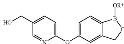
6-(1-hydroxy-1,3-dihydrobenzo[c][1,2]oxaborol-5-yloxy) nicotinaldehyde
