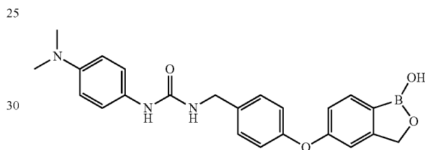
1-(4-Dimethylamino-phenyl)-3-[4-(1-hydroxy-1,3-dihydro-benzo[c][1,2]oxaborol-5-yloxy)-benzyl]-urea (D189)
