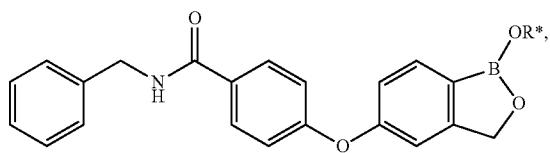
4-(1-Hydroxy-1,3-dihydro-benzo[c][1,2]oxaborol-5-yloxy)-N-(2-hydroxy-ethyl)-benzamide
