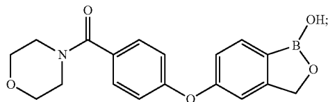
1,3-Dihydro-1-hydroxy-5-[4-(morpholinocarbonyl)phenoxy]-2,1-benzoxaborole
