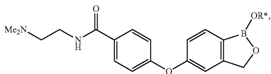
N-(2-Dimethylamino-ethyl)-4-(1-hydroxy-1,3-dihydro-benzo[c][1,2]oxaborol-5-yloxy)-benzamide
