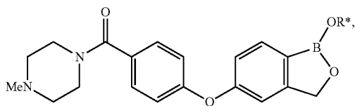
1-{4-[4-(1-Hydroxy-1,3-dihydro-benzo[c][1,2]oxaborol-5-yloxy)-benzoyl]-piperazin-1-yl}-ethanone
