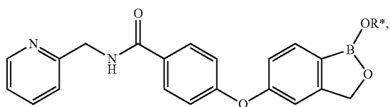
[4-(1-Hydroxy-1,3-dihydro-benzo[c][1,2]oxaborol-5-yloxy)-phenyl]-(4-methyl-piperazin-1-yl)-methanone
