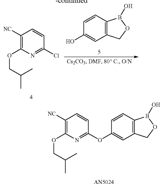
6-Chloro-2-isobutoxy-nicotinamide (3)
