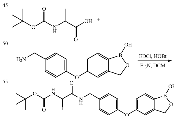
1-Cyclohexyl-3-[4-(1-hydroxy-1,3-dihydro-benzo[c][1,2]oxaborol-5-yloxy)-benzyl]-urea (D187)
