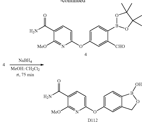
6-(4-Bromo-3-formyl-phenoxy)-2-methoxy-nicotinamide (3)
