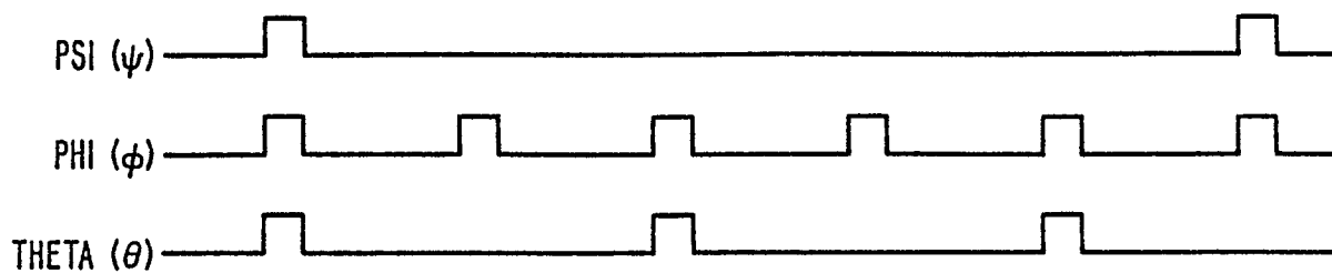
SYSTEM TIMING DIAGRAM
