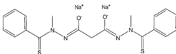
Compound (1)
