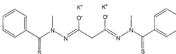
Compound (2)
