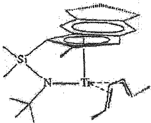
Chemical structure (IV)
