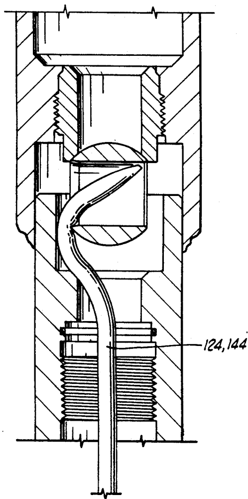
FIG. 9 PRIOR ART
