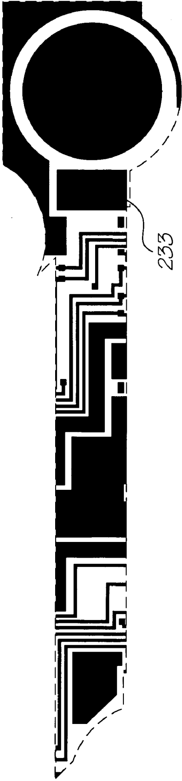
Metal 2 mask
