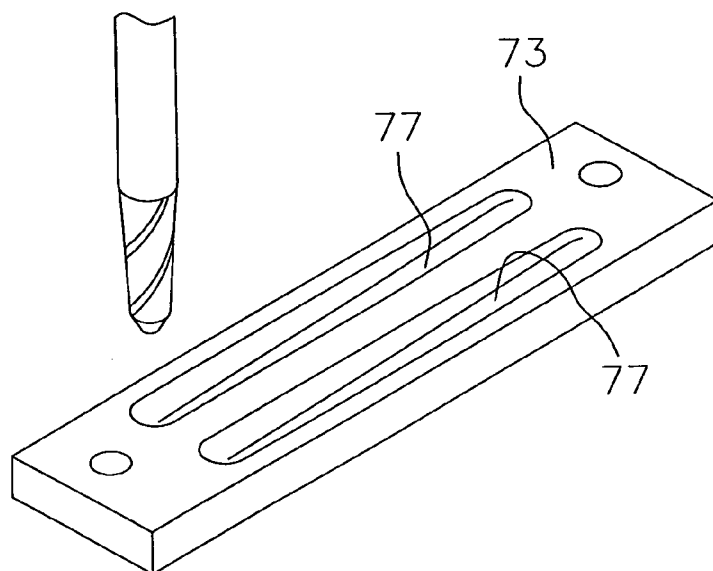
FIG. 7 PRIOR ART
