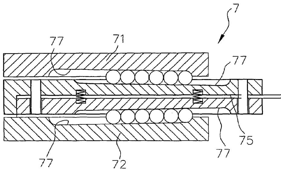
FIG. 6 PRIOR ART
