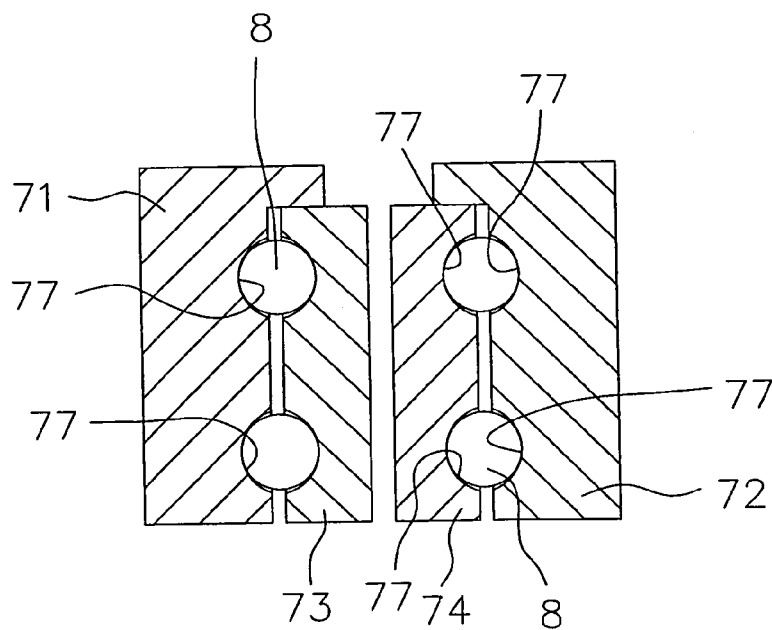
FIG. 8 PRIOR ART
