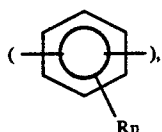
alkyl-substituted phenylene group
