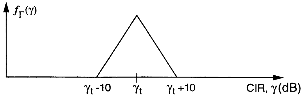
Example of probability density function (pdf) of the received CIR \gamma .
