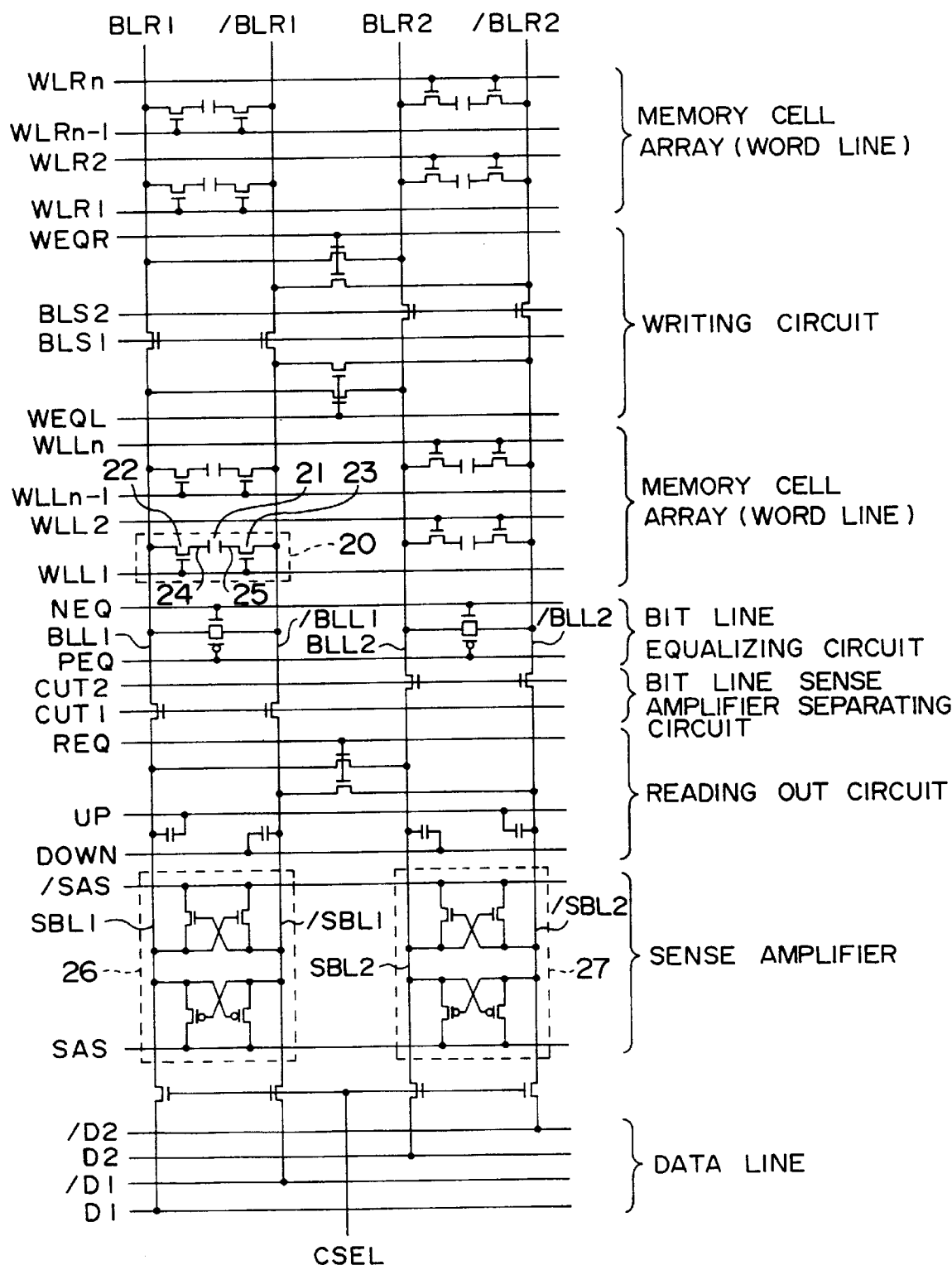
Fig. 10 PRIOR ART
