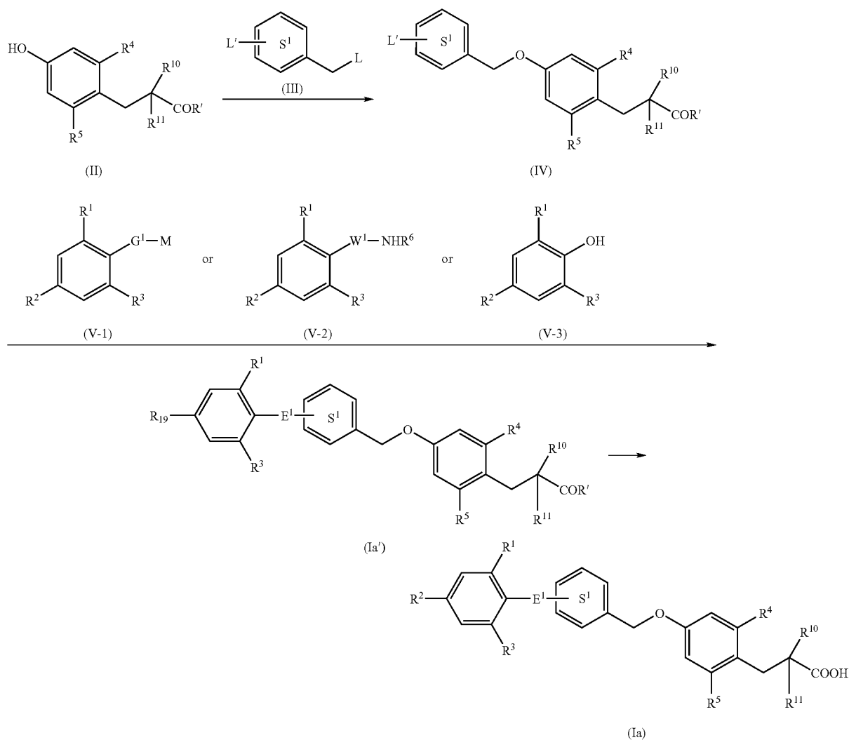
Reaction Scheme 1
