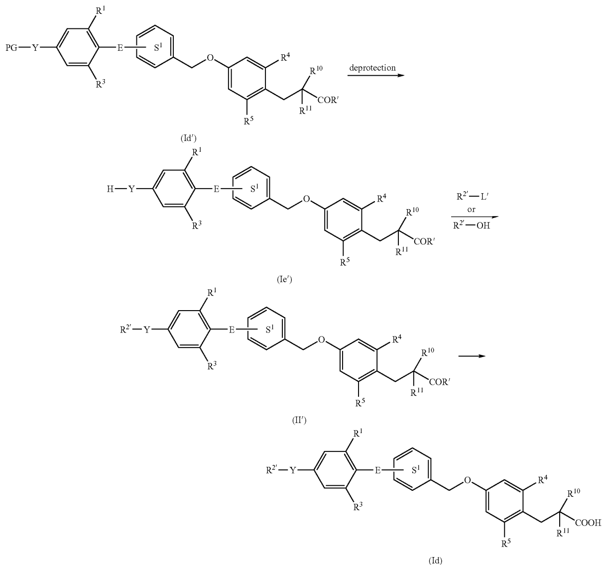
Reaction Scheme 4
