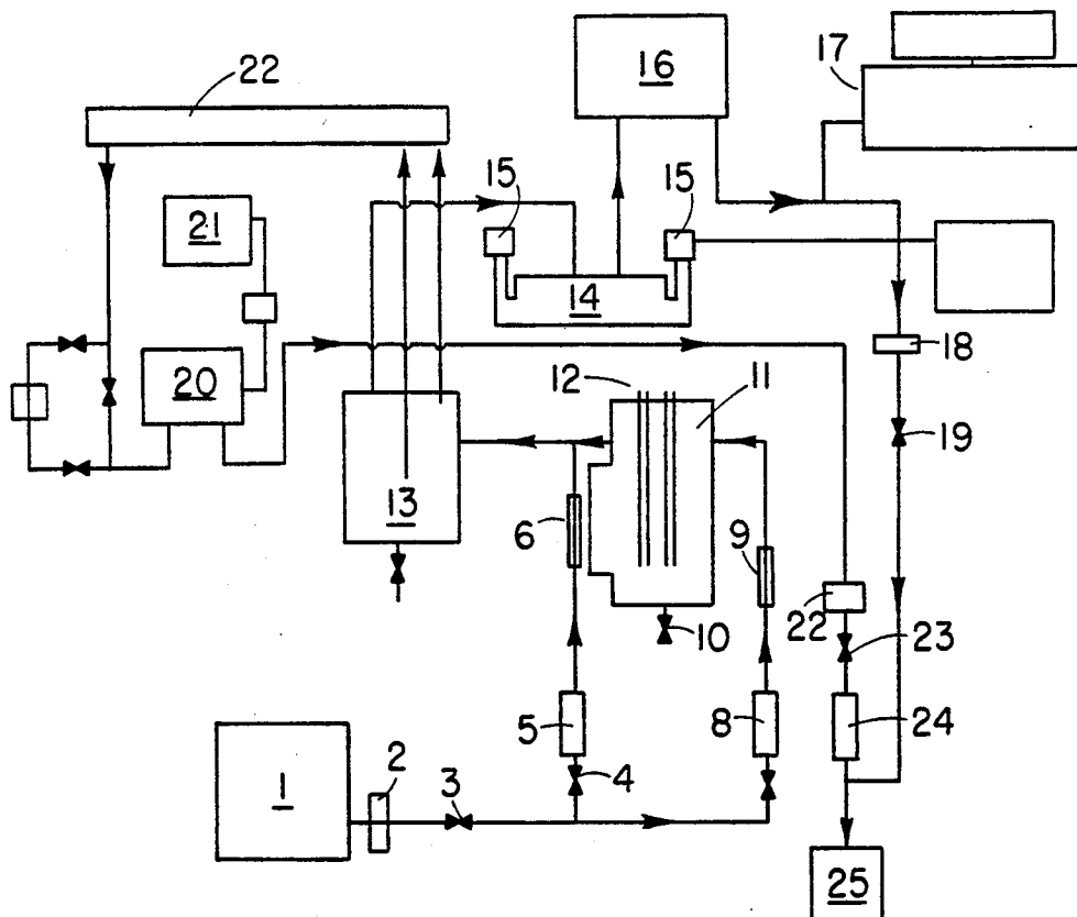
FLOW DIAGRAM TDA-100
