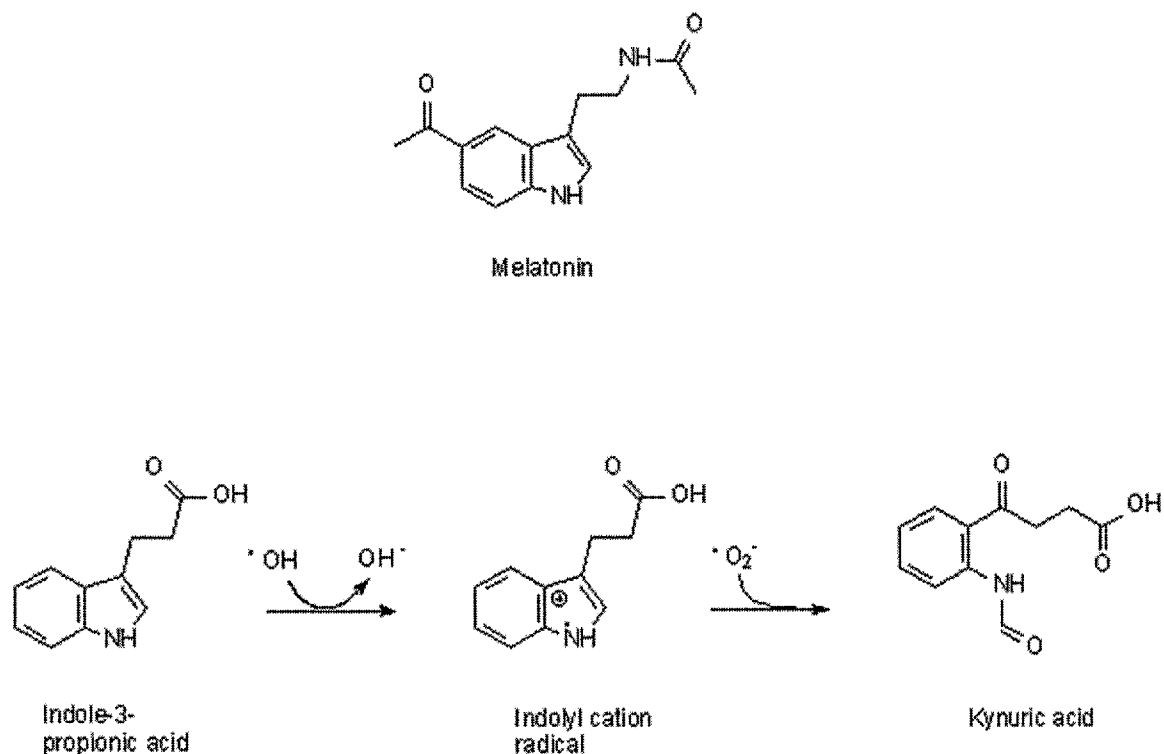
Mechanism of radical elimination by IPA
