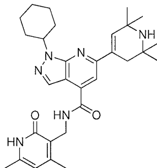
Compound B-16
