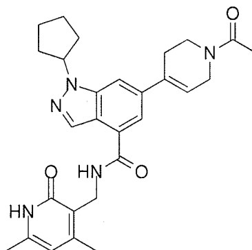
Compound D-4
