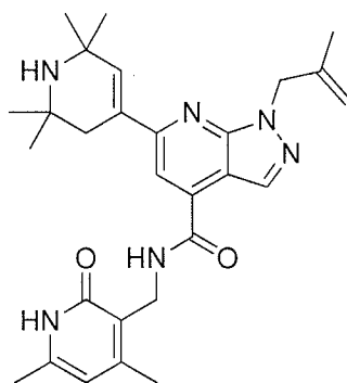
Compound B-3
