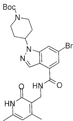
Compound D-12
