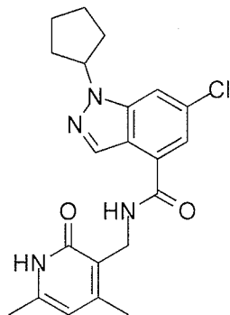
Compound D-10
