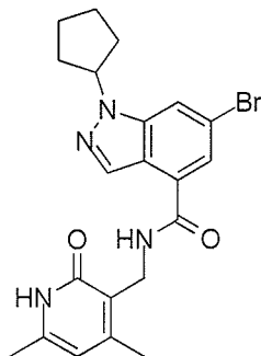
Compound D-1
