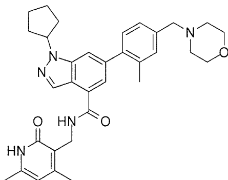
Compound C-6
