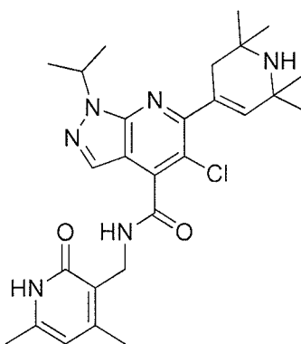
Compound B-12
