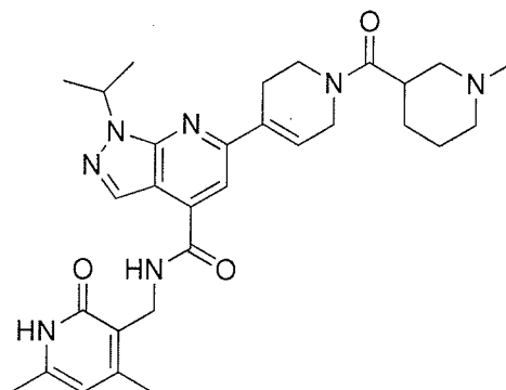
Compound B-32
