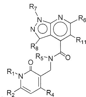
(IIc)
