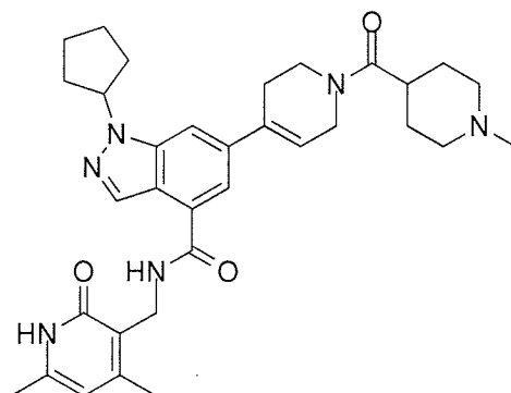
Compound D-5
