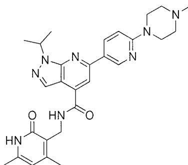
Compound A-11
