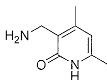
Compound C-1
