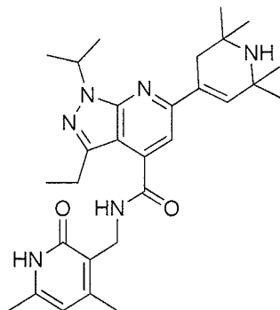
Compound B-26
