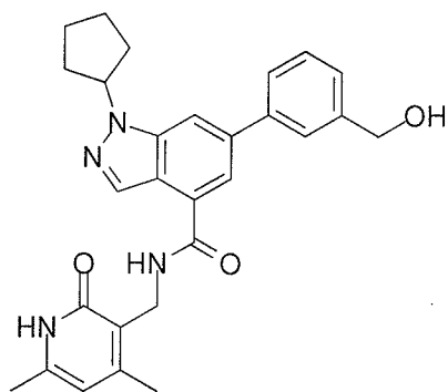
Compound C-8
