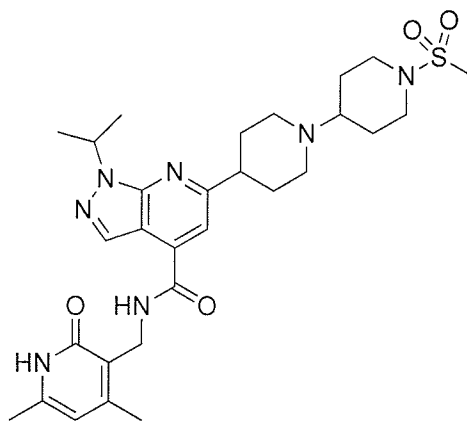
Compound B-35
