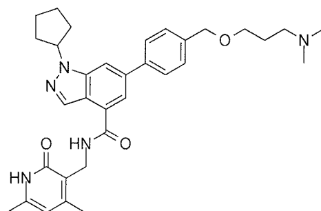
Compound C-4
