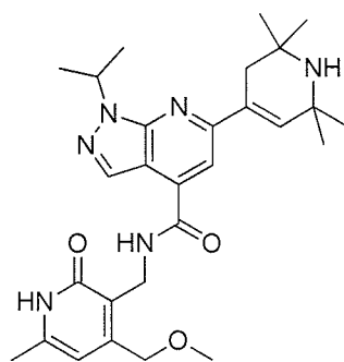
Compound B-21
