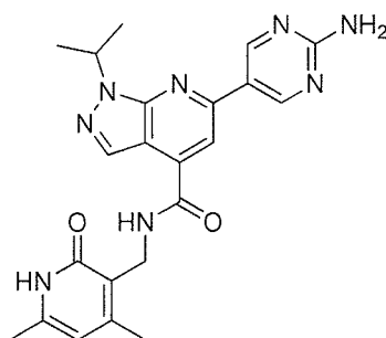
Compound A-4
