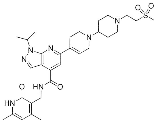
Compound B-33
