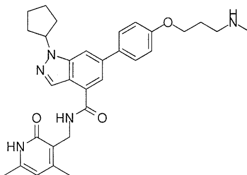
Compound C-12
