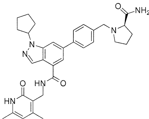
Compound C-13
