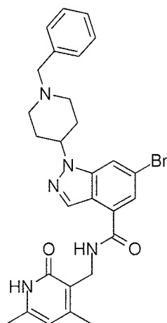
Compound D-15
