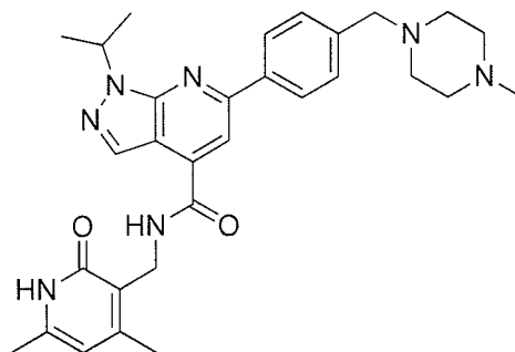
Compound A-8
