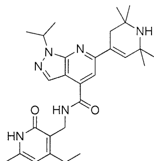
Compound B-25
