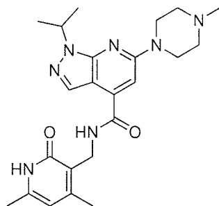
Compound B-9
