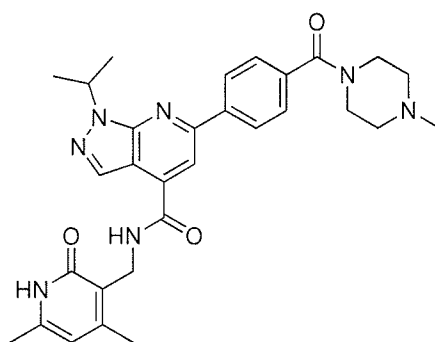
Compound A-12
