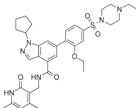
Compound C-14
