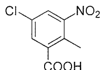
Compound D-10
