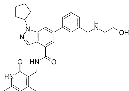
C-Compound 9
