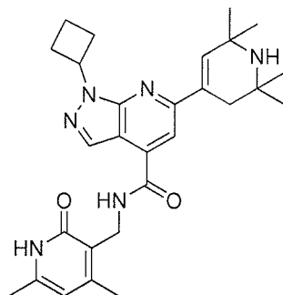
Compound B-14
