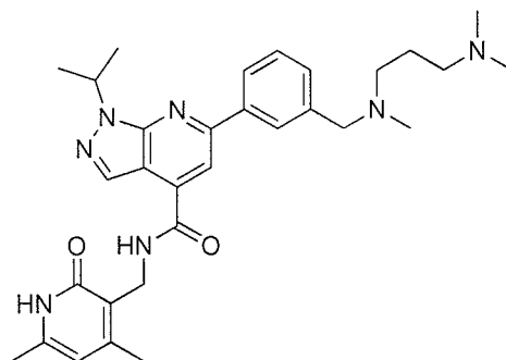
Compound A-16
