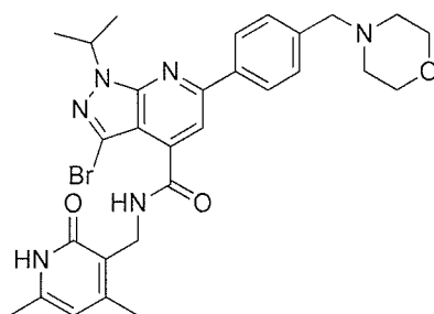
Compound A-17
