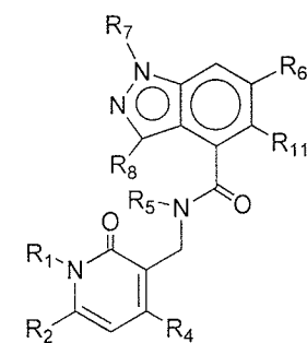
(IIIc)
