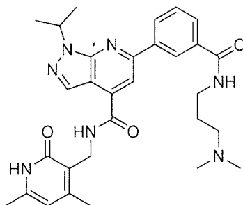
Compound A-13
