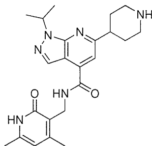
Compound B-24
