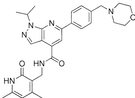
Compound A-2
