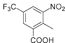
Compound D-11
