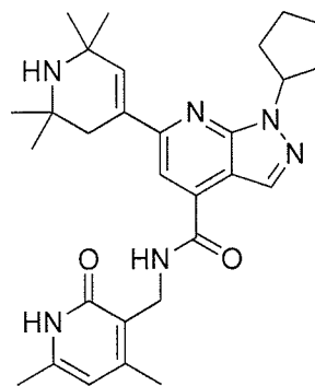
Compound B-5
