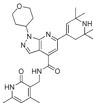
Compound B-10
