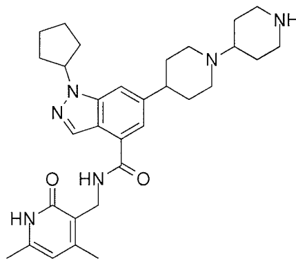
Compound D-6
