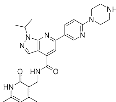
Compound A-10
