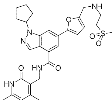
Compound C-7
