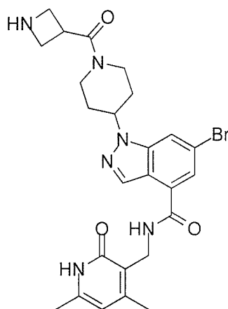
Compound D-14
