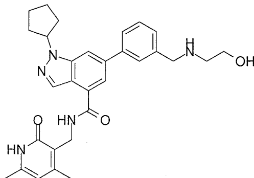
Compound C-9
