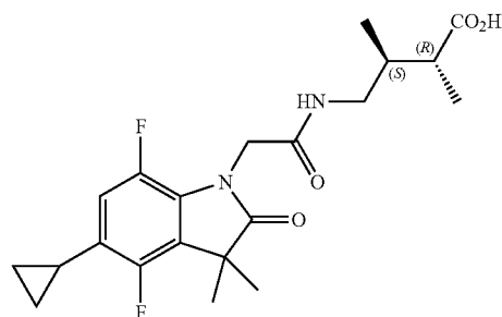
Compound 70D* (2R,3S)-4-(2-(5-cyclopropyl-4-7- difluoro-3,3-dimethyl-2-oxoindolin- 1-yl)acetamido)-2,3- dimethylbutanoic acid
