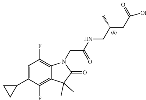
Compound 61A (R)-4-(2-(5-cyclopropyl-4,7-difluoro-3,3-dimethyl-2-oxoindolin-1-yl)acetamido)-3-methylbutanoic acid
