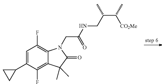
Compound 70-OMe* (assumed R/S and S/R mixture) of 70C*-OMe and 70D*-OMe)
