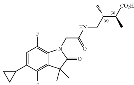
Compound 70C* (2S,3R)-4-(2-(5-cyclopropyl-4-7- difluoro-3,3-dimethyl-2-oxoindolin- 1-yl)acetamido)-2,3- dimethylbutanoic acid
