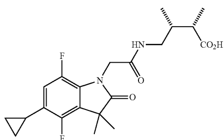
Compound 70* (assumed R/S and S/R mixture)
