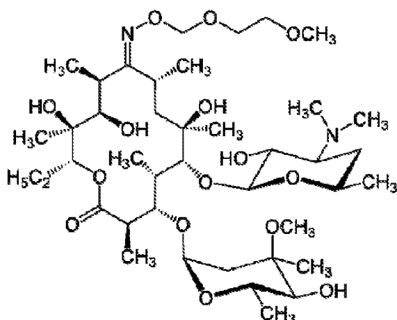
Roxithromycin
