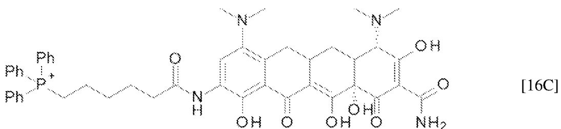
Tigecycline-TPP Conjugate
