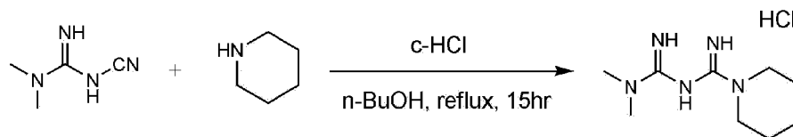
[Reaction Scheme 1]
