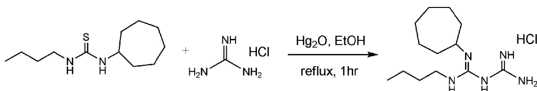
[Reaction Scheme 2]
