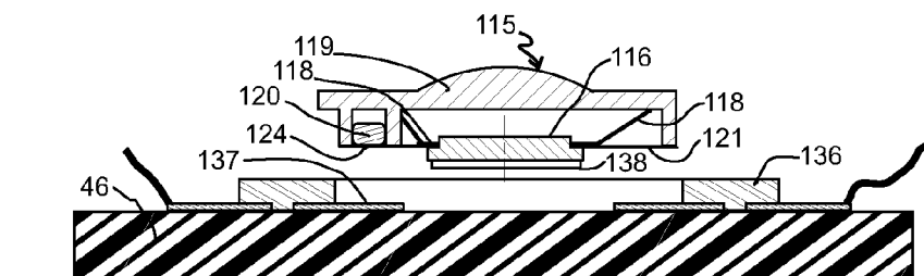
SECTION A-A (UNASSEMBLED)
