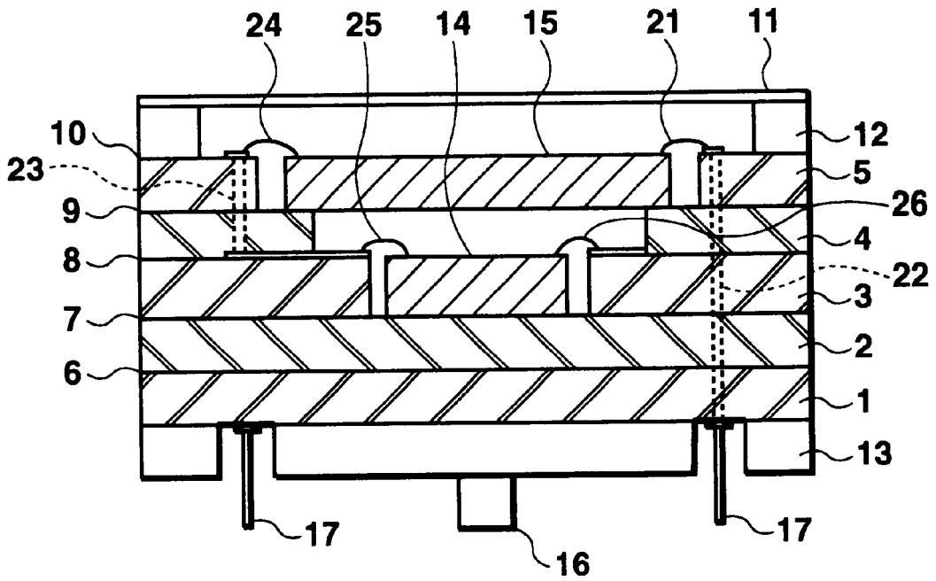
Fig. 17 PRIOR ART
