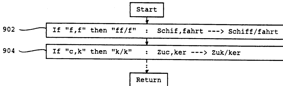
Figure 9 Special Soft Hyphen Processing for German Words
