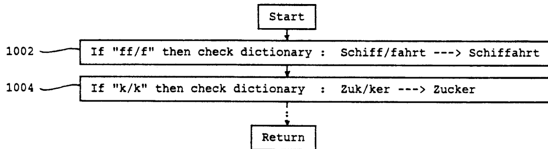
Figure 10 Dehyphenation for Hyphenated Special Processing German Words
