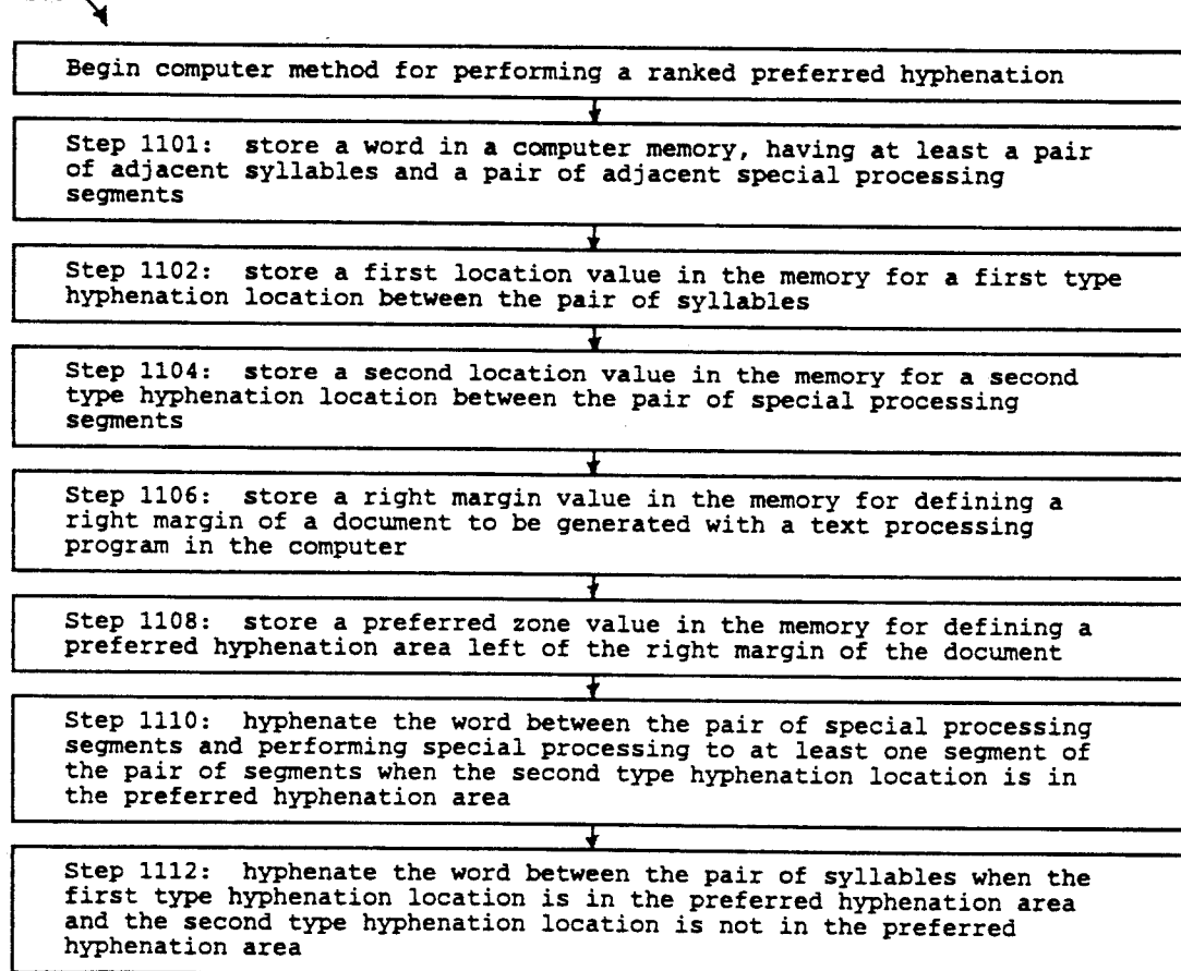
Figure 11 Flow Diagram of Preferred Ranked Special Processing Hyphenation
