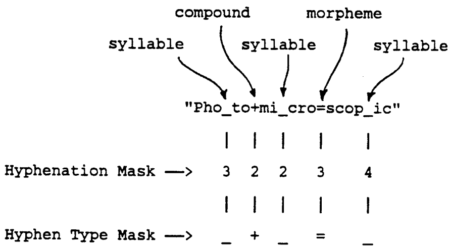
Figure 3 Example of Three Types of Soft Hyphenation
