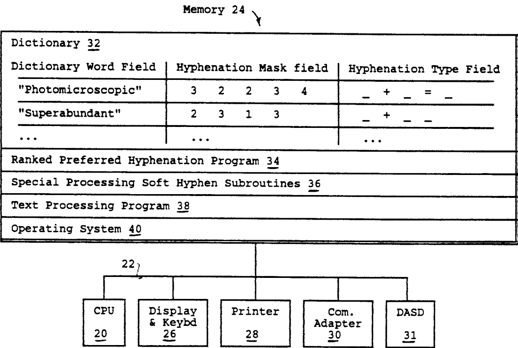
Figure 1 Text Processing System with Ranked Preferred Hyphenation
