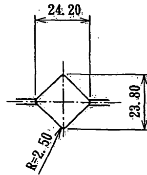
(2) Second pass caliber: square
