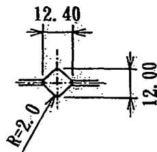
(4) Fourth pass caliber: square
