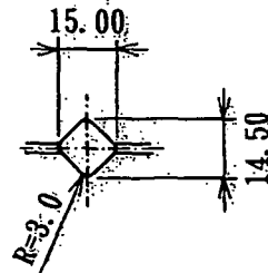
(2) Second pass caliber: square
