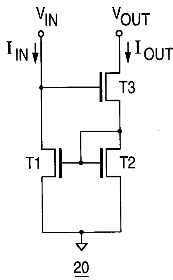
FIG. 2 (PRIOR ART)
