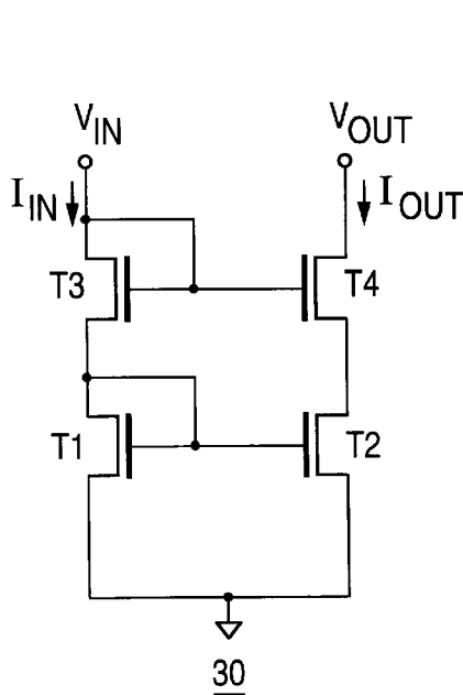
FIG. 3 (PRIOR ART)
