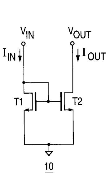
FIG. 1 (PRIOR ART)
