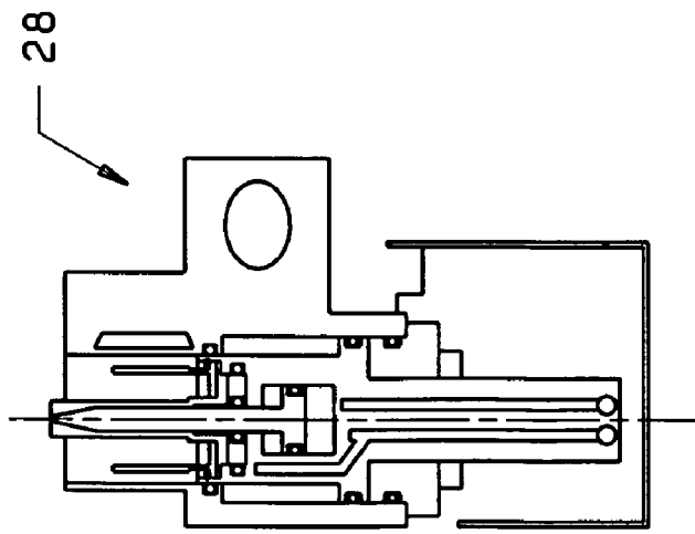
FINGERS RETRACTED
