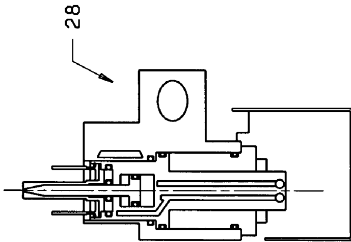
FINGERS EXTENDED
