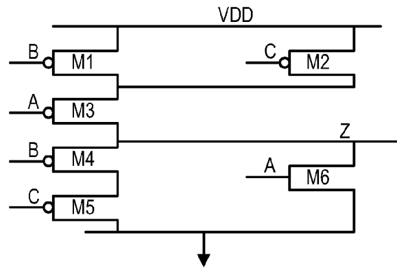
(a) 2-1 AO1 Gate z = A \& (B \mid C)
