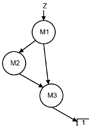
(a) DD For 2-1 AO1 z = A \& (B \mid C)
