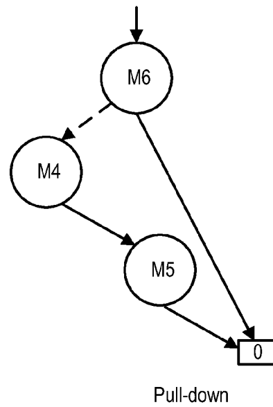
(b) DD for Pull-up and Pull-down paths
