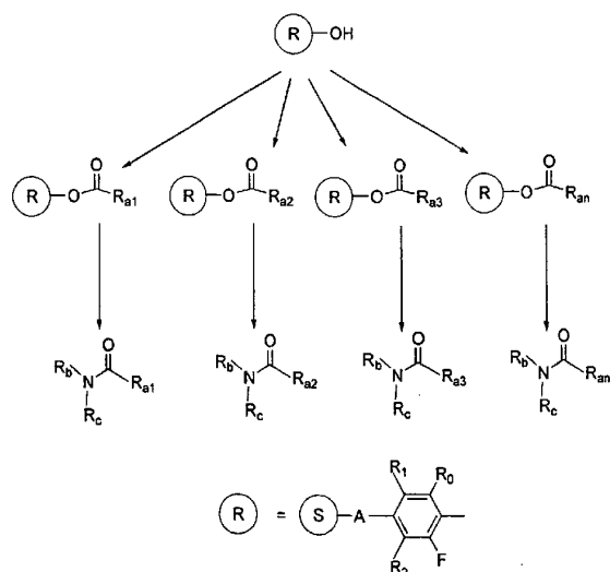
Scheme 14a
