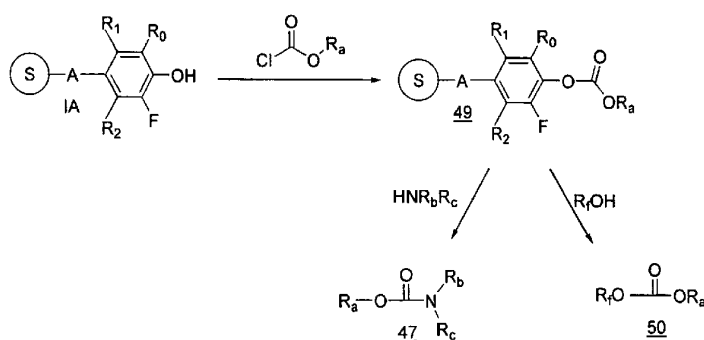
Scheme 12
