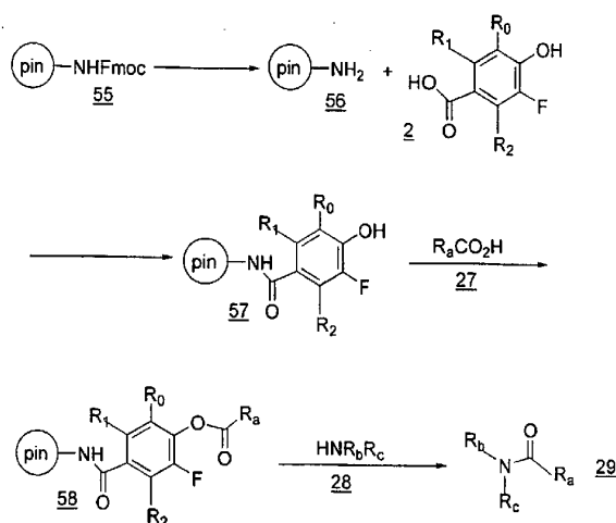
Scheme 16
