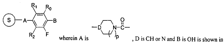
Scheme 2.
