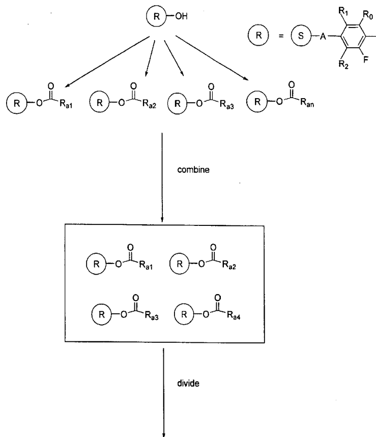
Scheme 15
