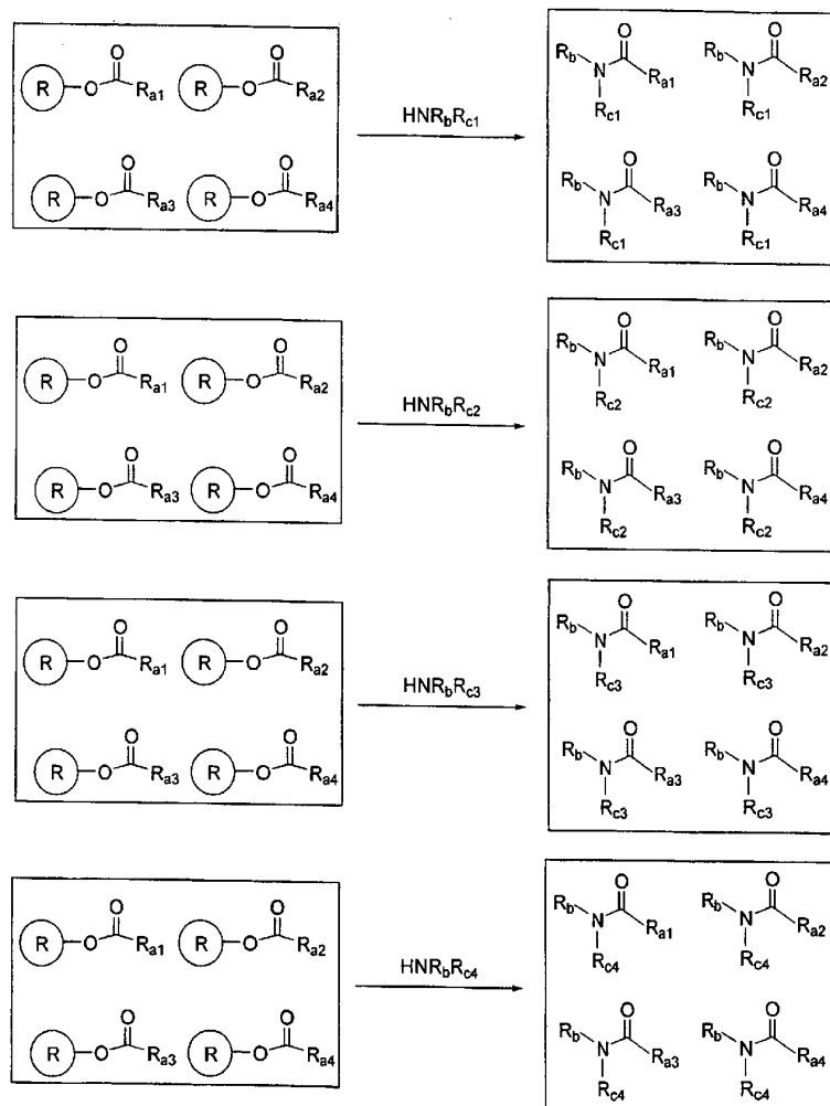
Scheme 15, cont.
