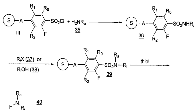
Scheme 9b
