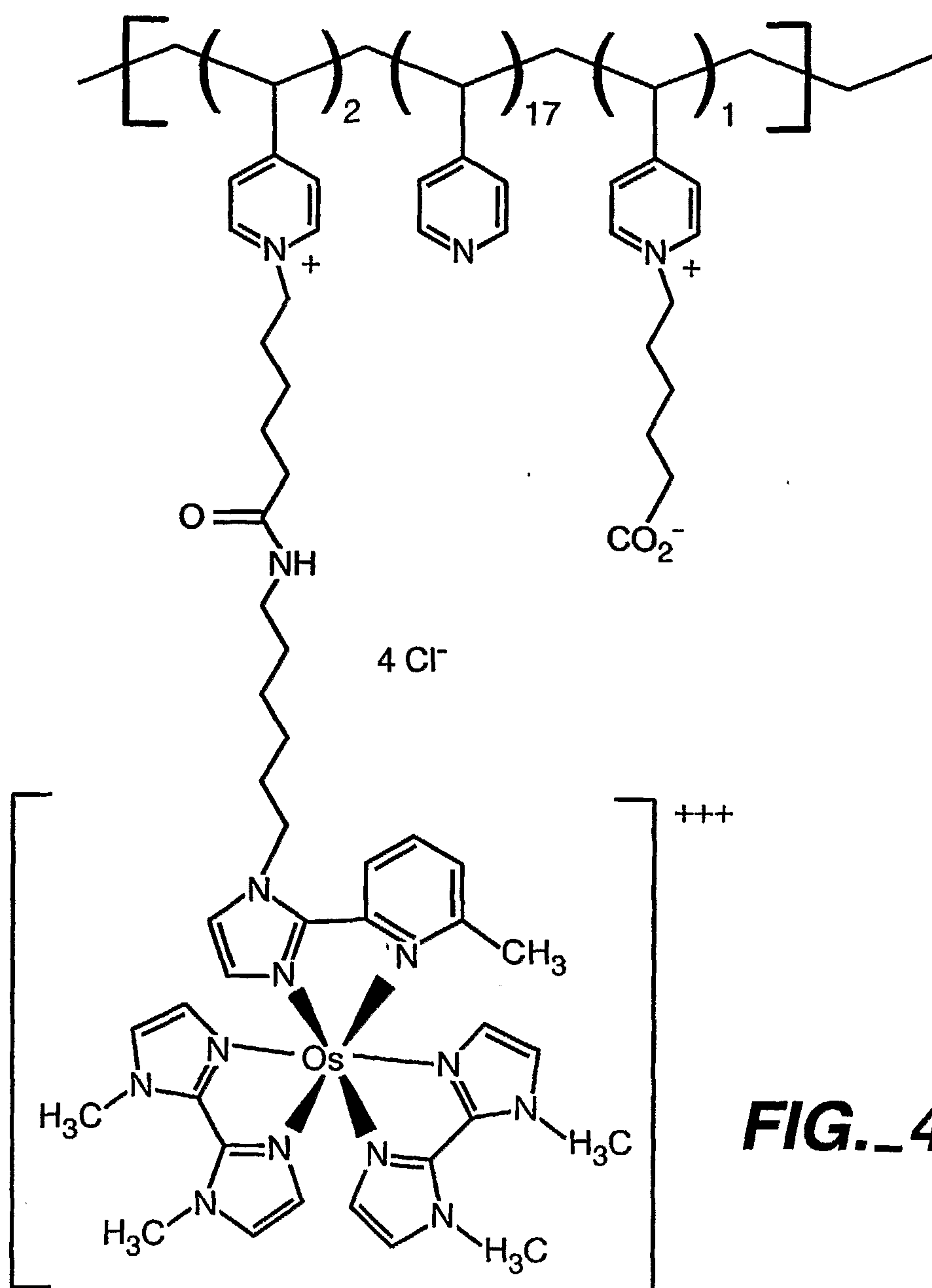
Structure of Redox Polymer 316
